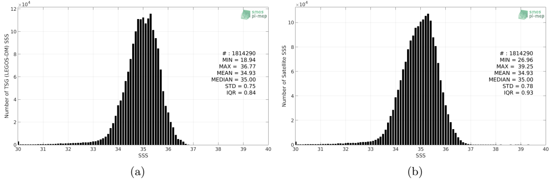
Figure 2: Histograms of SSS from TSG (LEGOS-DM) (a) and SMOS SSS L3 v4 - 9 Days (CATDS-CECOS-LOCEAN) (b) considering all match-up pairs per bins of 0.1 over the Pacific Ocean Pi-MEP region and for the full satellite product period.
