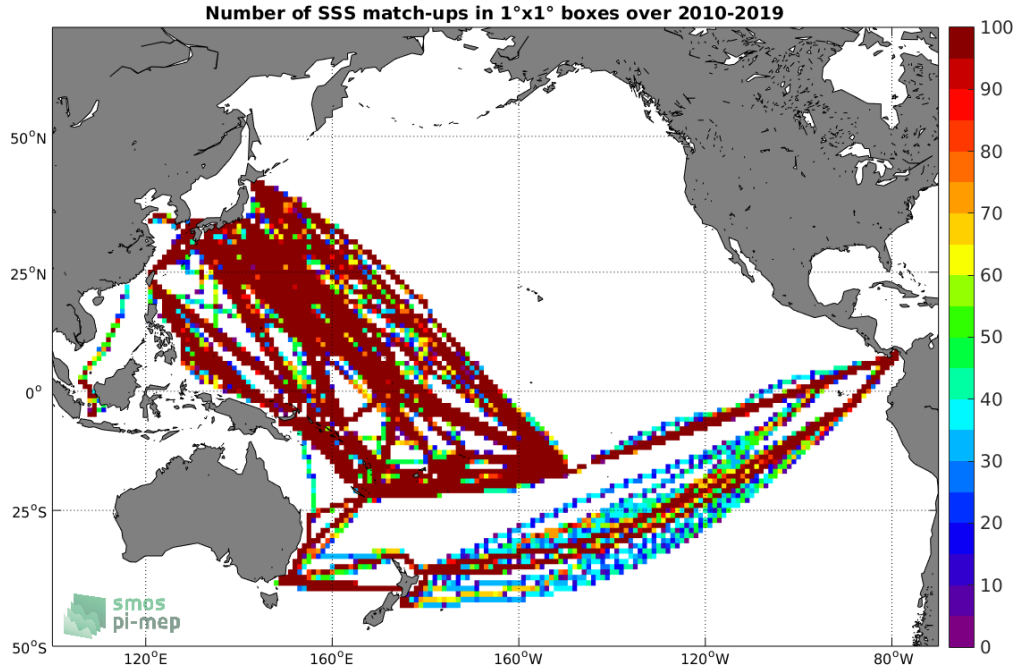
Figure 4: Number of SSS match-ups between TSG (LEGOS-DM) SSS and the SMOS SSS L3 v4 - 9 Days (CATDS-CECOS-LOCEAN) SSS product for the Pacific Ocean Pi-MEP region over 1°x1° boxes and for the full satellite product period.
