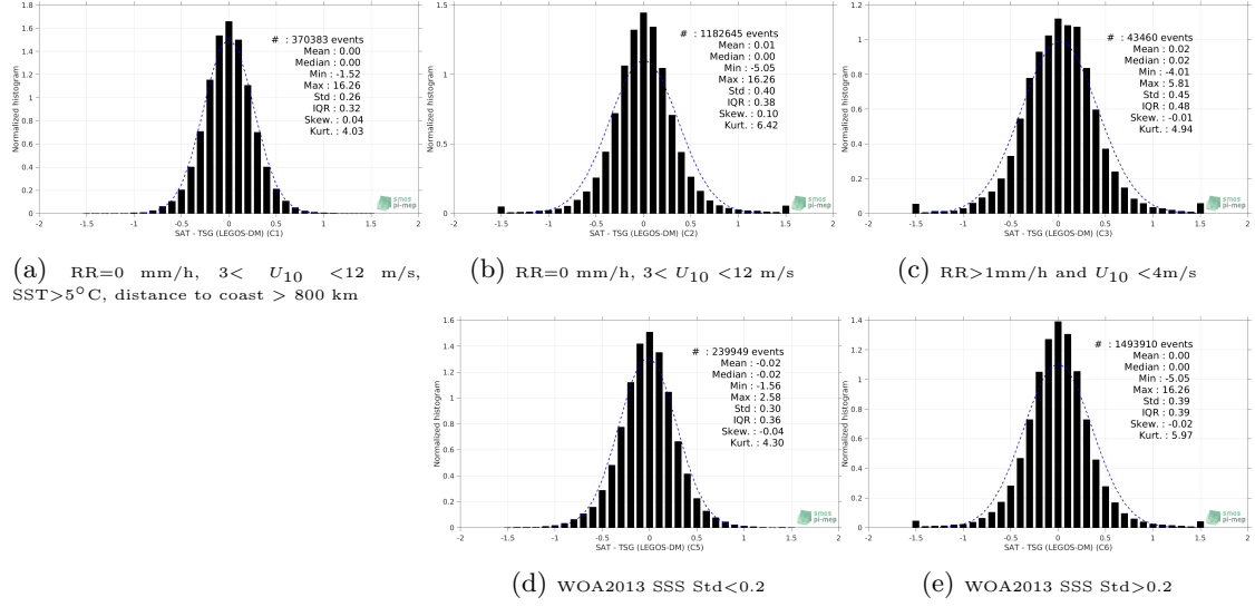
Figure 13: Normalized histogram of \Delta\text{SSS} (SMOS SSS L3 v4 - 9 Days (CATDS-CECOS-LOCEAN) - TSG (LEGOS-DM)) for 5 different subdatasets corresponding to: RR=0 mm/h, 3 < U_{10} < 12 m/s, SST > 5^\circ\text{C} , distance to coast > 800 km (a), RR=0 mm/h, 3 < U_{10} < 12 m/s (b), RR > 1\text{mm/h} and U_{10} < 4\text{m/s} (c), WOA2013 SSS Std < 0.2 (d), WOA2013 SSS Std > 0.2 (e).
