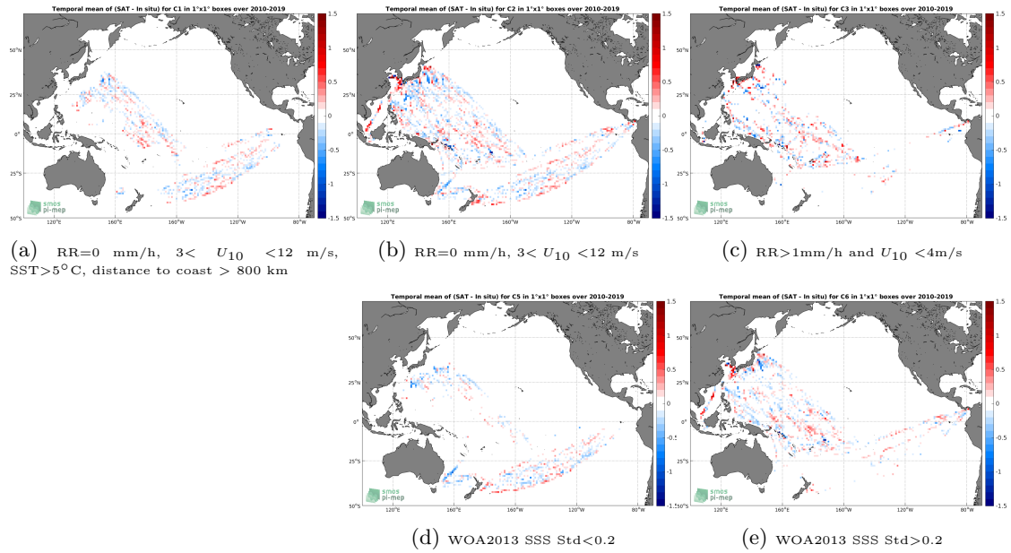
Figure 12: Temporal mean gridded over spatial boxes of size 1^\circ \times 1^\circ of \Delta SSS (SMOS SSS L3 v4 - 9 Days (CATDS-CECOS-LOCEAN) - TSG (LEGOS-DM)) for 5 different subdatasets corresponding to: RR=0 mm/h, 3 < U_{10} < 12 m/s, SST > 5^\circ\text{C} , distance to coast > 800 km (a), RR=0 mm/h, 3 < U_{10} < 12 m/s (b), RR > 1 mm/h and U_{10} < 4 m/s (c), WOA2013 SSS Std < 0.2 (d), WOA2013 SSS Std > 0.2 (e).
