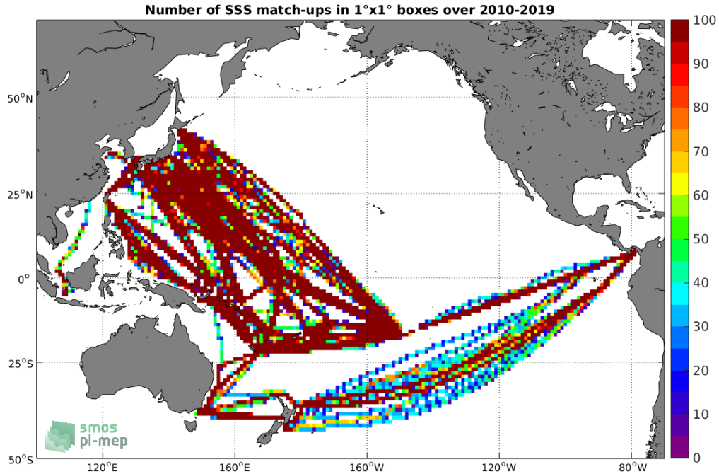
Figure 4: Number of SSS match-ups between TSG-LEGOS-DM SSS and the SMOS-L3-CATDS-CECOS-LOCEAN-V4-9DAYS-25KM SSS product for the Pacific Ocean Pi-MEP region over 1°x1° boxes and for the full satellite product period.
