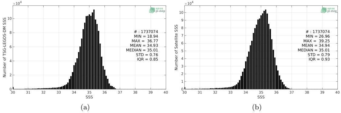
Figure 2: Histograms of SSS from TSG-LEGOS-DM (a) and SMOS-L3-CATDS-CECOS-LOCEAN-V4-9DAYS-25KM (b) considering all match-up pairs per bins of 0.1 over the Pacific Ocean Pi-MEP region and for the full satellite product period.
