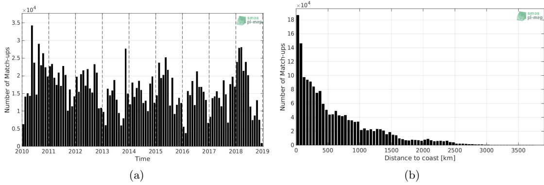
Figure 1: Number of match-ups between TSG-LEGOS-DM and SMOS-L3-CATDS-CECOS-LOCEAN-V4-9DAYS-25KM SSS as a function of time (a) and as function of the distance to coast (b) over the Pacific Ocean Pi-MEP region and for the full satellite product period.
