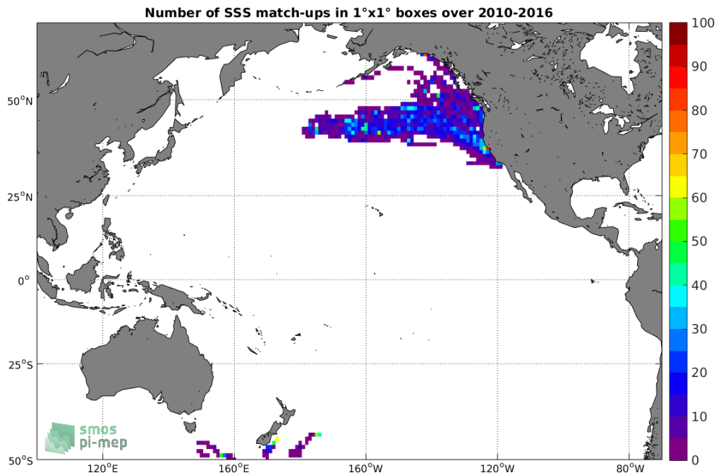
Figure 4: Number of SSS match-ups between Sea mammals SSS and the SMOS SSS L3 v4 - 9 Days (CATDS-CECOS-LOCEAN) SSS product for the Pacific Ocean Pi-MEP region over 1°x1° boxes and for the full satellite product period.
