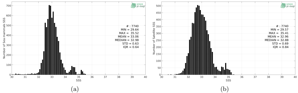
Figure 2: Histograms of SSS from Sea mammals (a) and SMOS SSS L3 v4 - 9 Days (CATDS-CECOS-LOCEAN) (b) considering all match-up pairs per bins of 0.1 over the Pacific Ocean Pi-MEP region and for the full satellite product period.
