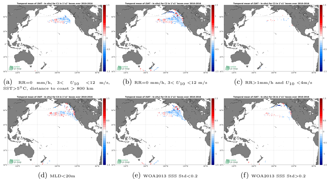
Figure 12: Temporal mean gridded over spatial boxes of size 1^\circ \times 1^\circ of \Delta SSS (SMOS SSS L3 v4 - 9 Days (CATDS-CECOS-LOCEAN) - Sea mammals) for 6 different subdatasets corresponding to:RR=0 mm/h, 3 < U_{10} < 12 m/s, SST > 5^\circ\text{C} , distance to coast > 800 km (a), RR=0 mm/h, 3 < U_{10} < 12 m/s (b), RR > 1 mm/h and U_{10} < 4 m/s (c),MLD < 20 m (d),WOA2013 SSS Std < 0.2 (e),WOA2013 SSS Std > 0.2 (f).
