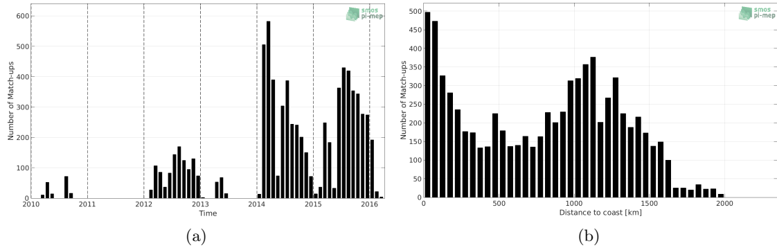
Figure 1: Number of match-ups between Sea mammals and SMOS SSS L3 v4 - 9 Days (CATDS-CECOS-LOCEAN) SSS as a function of time (a) and as function of the distance to coast (b) over the Pacific Ocean Pi-MEP region and for the full satellite product period.
