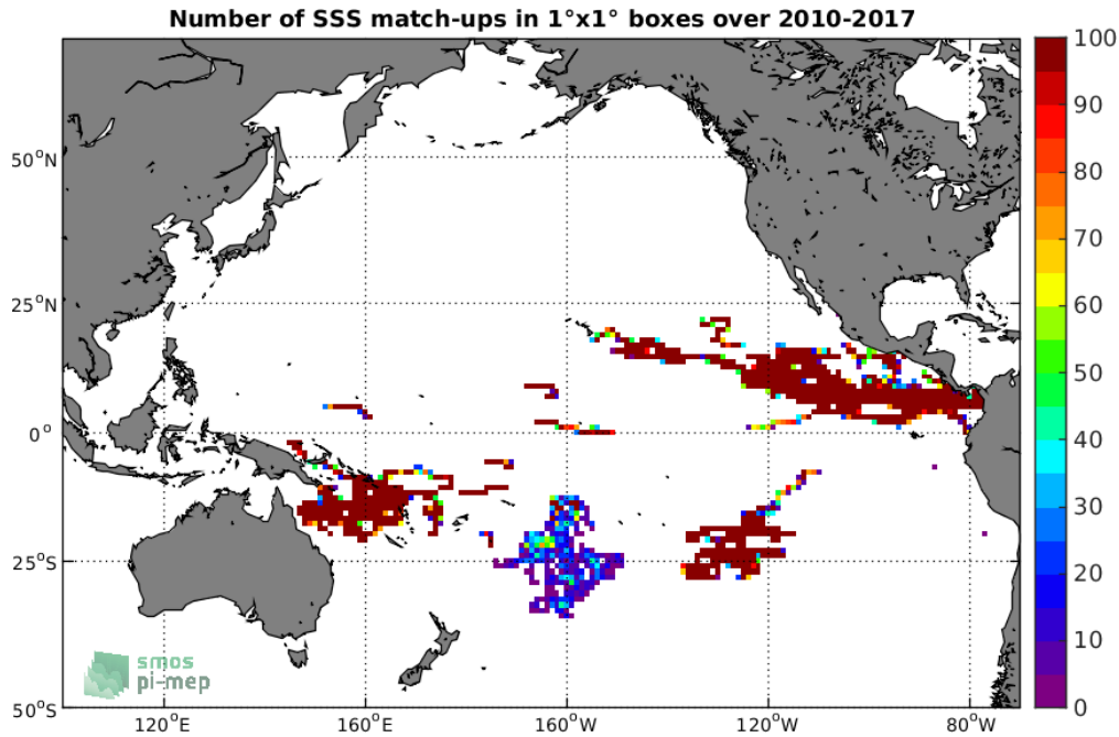
Figure 3: Number of SSS match-ups between Surface drifters SSS and the SMOS-L3-CATDS-CECOS-LOCEAN-V4-9DAYS-25KM SSS product for the Pacific Ocean Pi-MEP region over 1^\circ \times 1^\circ boxes and for the full satellite product period.
