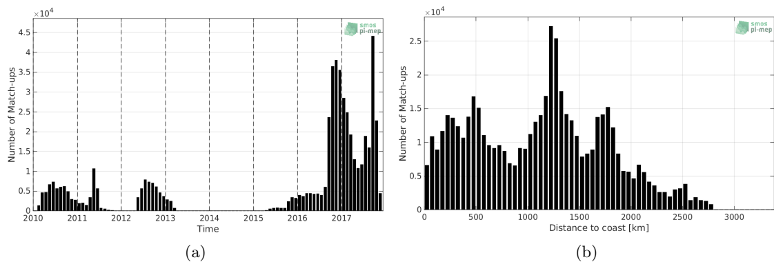
Figure 1: Number of match-ups between Surface drifters and SMOS-L3-CATDS-CECOS-LOCEAN-V4-9DAYS-25KM SSS as a function of time (a) and as function of the distance to coast (b) over the Pacific Ocean Pi-MEP region and for the full satellite product period.
