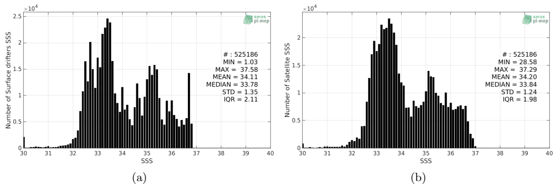
Figure 2: Histograms of SSS from Surface drifters (a) and SMOS-L3-CATDS-CECOS-LOCEAN-V4-9DAYS-25KM (b) considering all match-up pairs per bins of 0.1 over the Pacific Ocean Pi-MEP region and for the full satellite product period.
