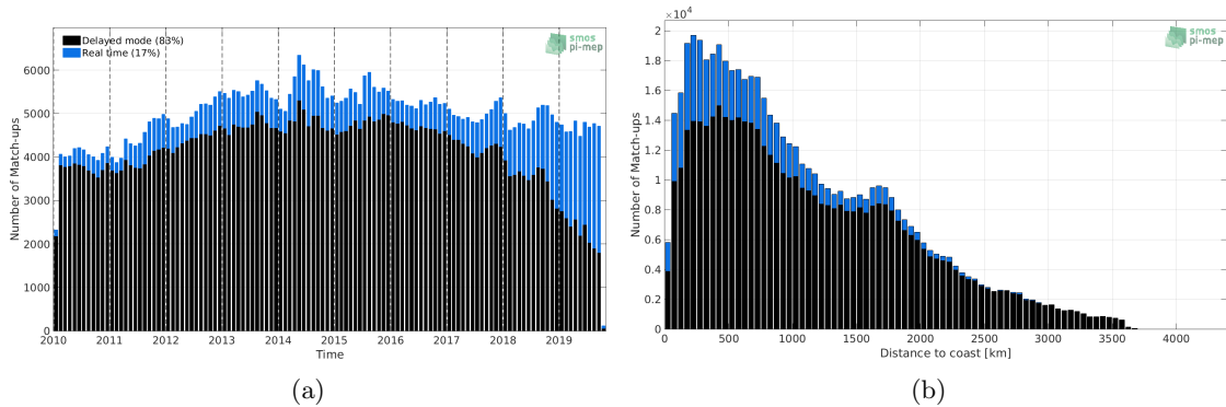
Figure 1: Number of match-ups between Argo and SMOS SSS L3 v4 - 9 Days (CATDS-CECOS-LOCEAN) SSS as a function of time (a) and as function of the distance to coast (b) over the Pacific Ocean Pi-MEP region and for the full satellite product period.
