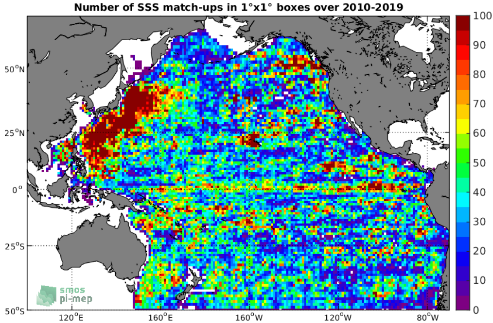
Figure 4: Number of SSS match-ups between Argo SSS and the SMOS-L3-CATDS-CECOS-LOCEAN-V4-9DAYS-25KM SSS product for the Pacific Ocean Pi-MEP region over 1°x1° boxes and for the full satellite product period.
