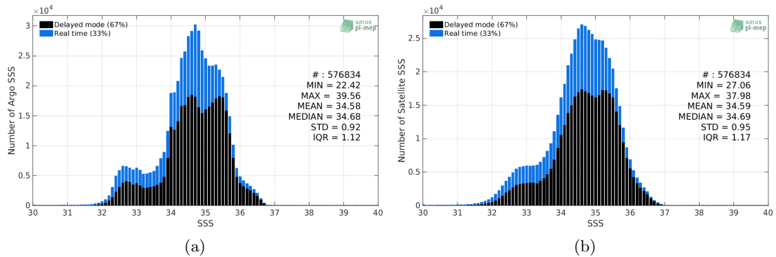
Figure 2: Histograms of SSS from Argo (a) and SMOS-L3-CATDS-CECOS-LOCEAN-V4-9DAYS-25KM (b) considering all match-up pairs per bins of 0.1 over the Pacific Ocean Pi-MEP region and for the full satellite product period.
