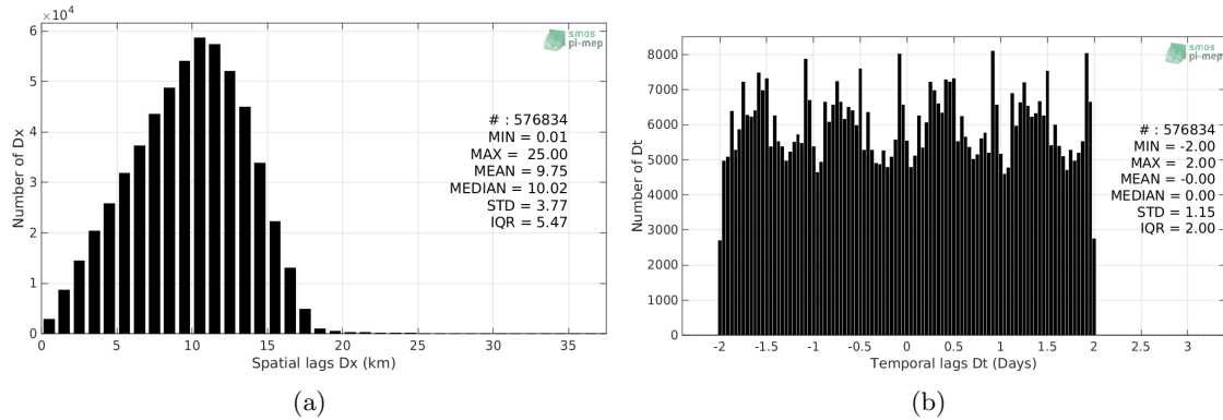
Figure 5: Histograms of the spatial (a) and temporal (b) lags between the time of the Argo measurements and the date of the corresponding SMOS-L3-CATDS-CECOS-LOCEAN-V4-9DAYS-25KM SSS product.
