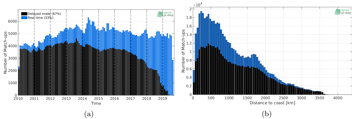
Figure 1: Number of match-ups between Argo and SMOS-L3-CATDS-CECOS-LOCEAN-V4-9DAYS-25KM SSS as a function of time (a) and as function of the distance to coast (b) over the Pacific Ocean Pi-MEP region and for the full satellite product period.
