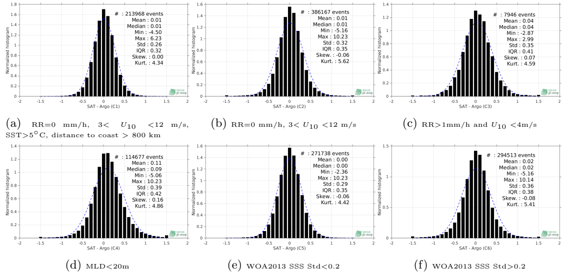
Figure 13: Normalized histogram of \Delta\text{SSS} (SMOS-L3-CATDS-CECOS-LOCEAN-V4-9DAYS-25KM - Argo) for 6 different subdatasets corresponding to: RR=0 mm/h, 3 < U_{10} < 12 m/s, SST>5°C, distance to coast > 800 km (a), RR=0 mm/h, 3 < U_{10} < 12 m/s (b), RR>1mm/h and U_{10} < 4 m/s (c), MLD<20m (d), WOA2013 SSS Std<0.2 (e), WOA2013 SSS Std>0.2 (f).
