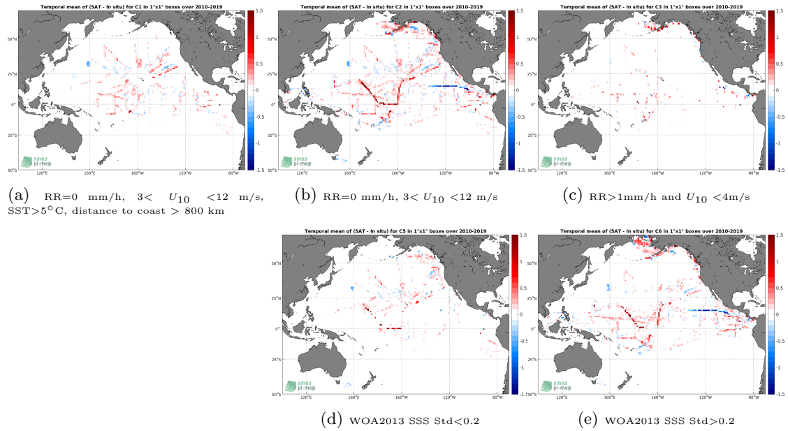
Figure 12: Temporal mean gridded over spatial boxes of size 1^\circ \times 1^\circ of \Delta SSS (SMOS SSS L3 v4 - 18 Days (CATDS-CECOS-LOCEAN) - TSG (SAMOS)) for 5 different subdatasets corresponding to: RR=0 mm/h, 3 < U_{10} < 12 m/s, SST > 5^\circ C , distance to coast > 800 km (a), RR=0 mm/h, 3 < U_{10} < 12 m/s (b), RR > 1 mm/h and U_{10} < 4 m/s (c), WOA2013 SSS Std < 0.2 (d), WOA2013 SSS Std > 0.2 (e).
