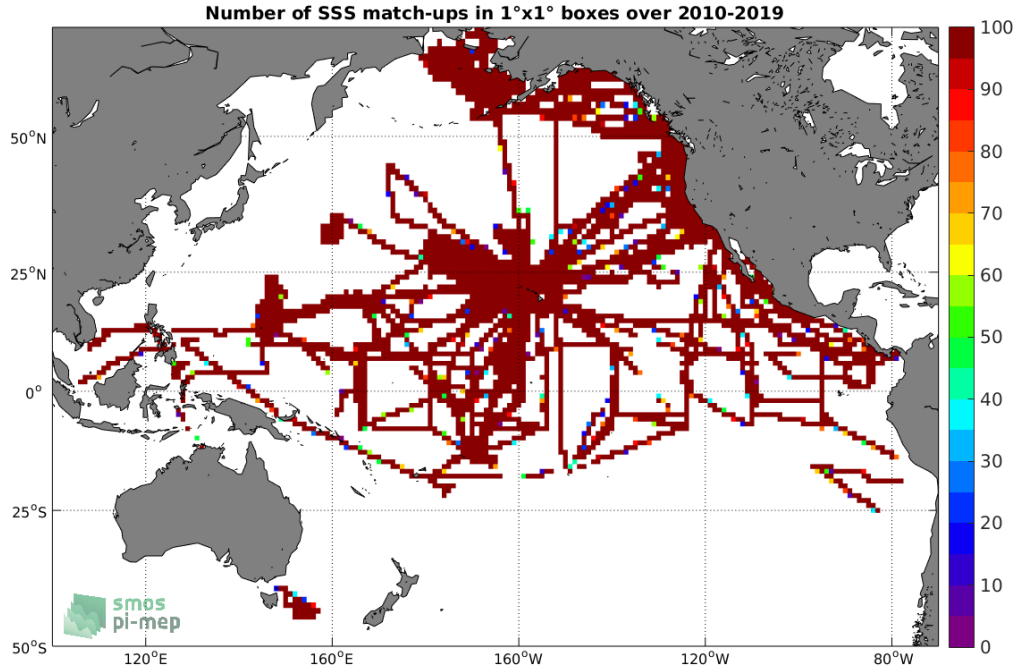
Figure 4: Number of SSS match-ups between TSG (SAMOS) SSS and the SMOS SSS L3 v4 - 18 Days (CATDS-CECOS-LOCEAN) SSS product for the Pacific Ocean Pi-MEP region over 1^\circ \times 1^\circ boxes and for the full satellite product period.
