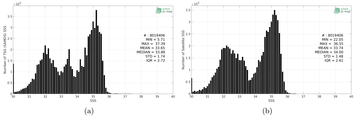
Figure 2: Histograms of SSS from TSG (SAMOS) (a) and SMOS SSS L3 v4 - 18 Days (CATDS-CECOS-LOCEAN) (b) considering all match-up pairs per bins of 0.1 over the Pacific Ocean Pi-MEP region and for the full satellite product period.
