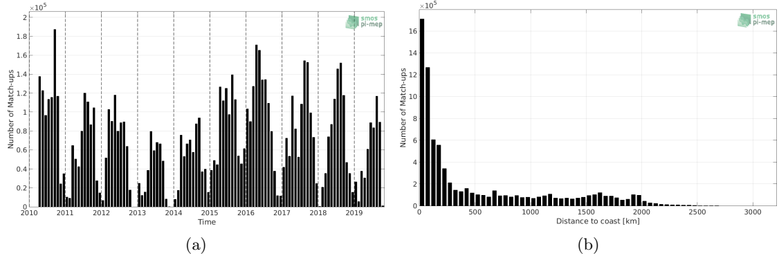
Figure 1: Number of match-ups between TSG (SAMOS) and SMOS SSS L3 v4 - 18 Days (CATDS-CECOS-LOCEAN) SSS as a function of time (a) and as function of the distance to coast (b) over the Pacific Ocean Pi-MEP region and for the full satellite product period.
