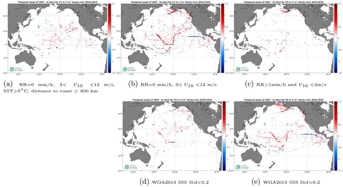
Figure 12: Temporal mean gridded over spatial boxes of size 1^\circ \times 1^\circ of \Delta SSS (SMOS-L3-CATDS-CECOS-LOCEAN-V4-18DAYS-25KM - TSG-SAMOS) for 5 different subdatasets corresponding to: RR=0 mm/h, 3 < U_{10} < 12 m/s, SST > 5^\circ C , distance to coast > 800 km (a), RR=0 mm/h, 3 < U_{10} < 12 m/s (b), RR > 1 mm/h and U_{10} < 4 m/s (c), WOA2013 SSS Std < 0.2 (d), WOA2013 SSS Std > 0.2 (e).
