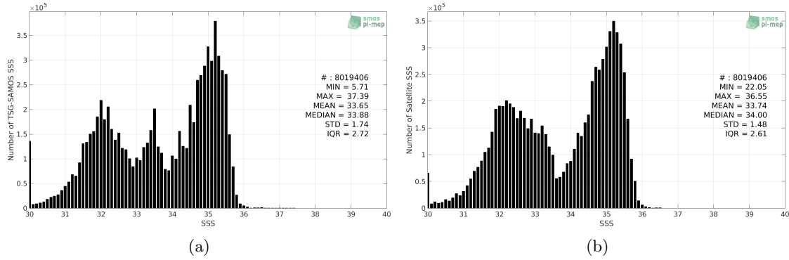
Figure 2: Histograms of SSS from TSG-SAMOS (a) and SMOS-L3-CATDS-CECOS-LOCEAN-V4-18DAYS-25KM (b) considering all match-up pairs per bins of 0.1 over the Pacific Ocean Pi-MEP region and for the full satellite product period.
