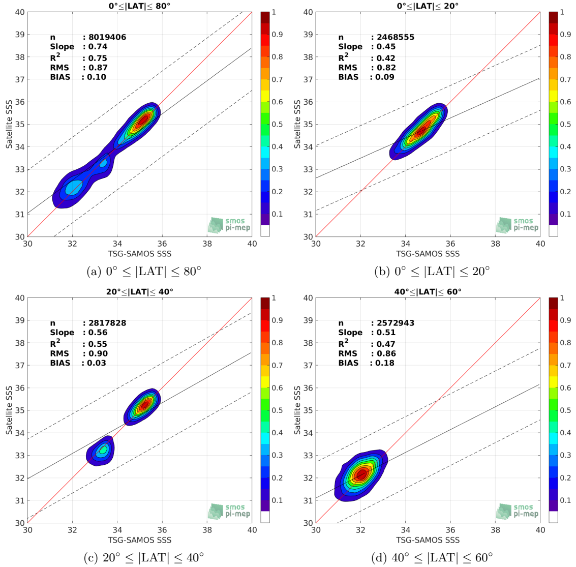
Figure 9: Contour maps of the concentration of SMOS-L3-CATDS-CECOS-LOCEAN-V4-18DAYS-25KM SSS (y-axis) versus TSG-SAMOS SSS (x-axis) at match-up pairs for different latitude bands. For each plot, the red line shows x=y . The black thin and dashed lines indicate a linear fit through the data cloud and the \pm 95\% confidence levels, respectively. The number match-up pairs n , the slope and R^2 coefficient of the linear fit, the root mean square (RMS) and the mean bias between satellite and in situ data are indicated for each latitude band in each plots.
