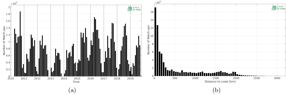
Figure 1: Number of match-ups between TSG-SAMOS and SMOS-L3-CATDS-CECOS-LOCEAN-V4-18DAYS-25KM SSS as a function of time (a) and as function of the distance to coast (b) over the Pacific Ocean Pi-MEP region and for the full satellite product period.
