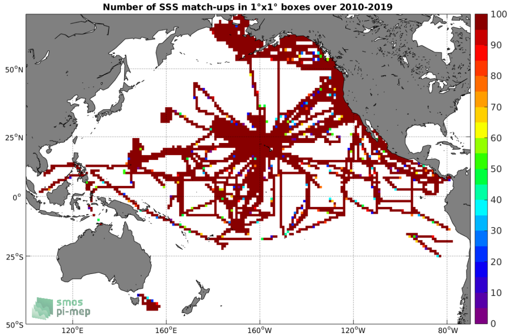
Figure 4: Number of SSS match-ups between TSG-SAMOS SSS and the SMOS-L3-CATDS-CECOS-LOCEAN-V4-18DAYS-25KM SSS product for the Pacific Ocean Pi-MEP region over 1^\circ \times 1^\circ boxes and for the full satellite product period.
