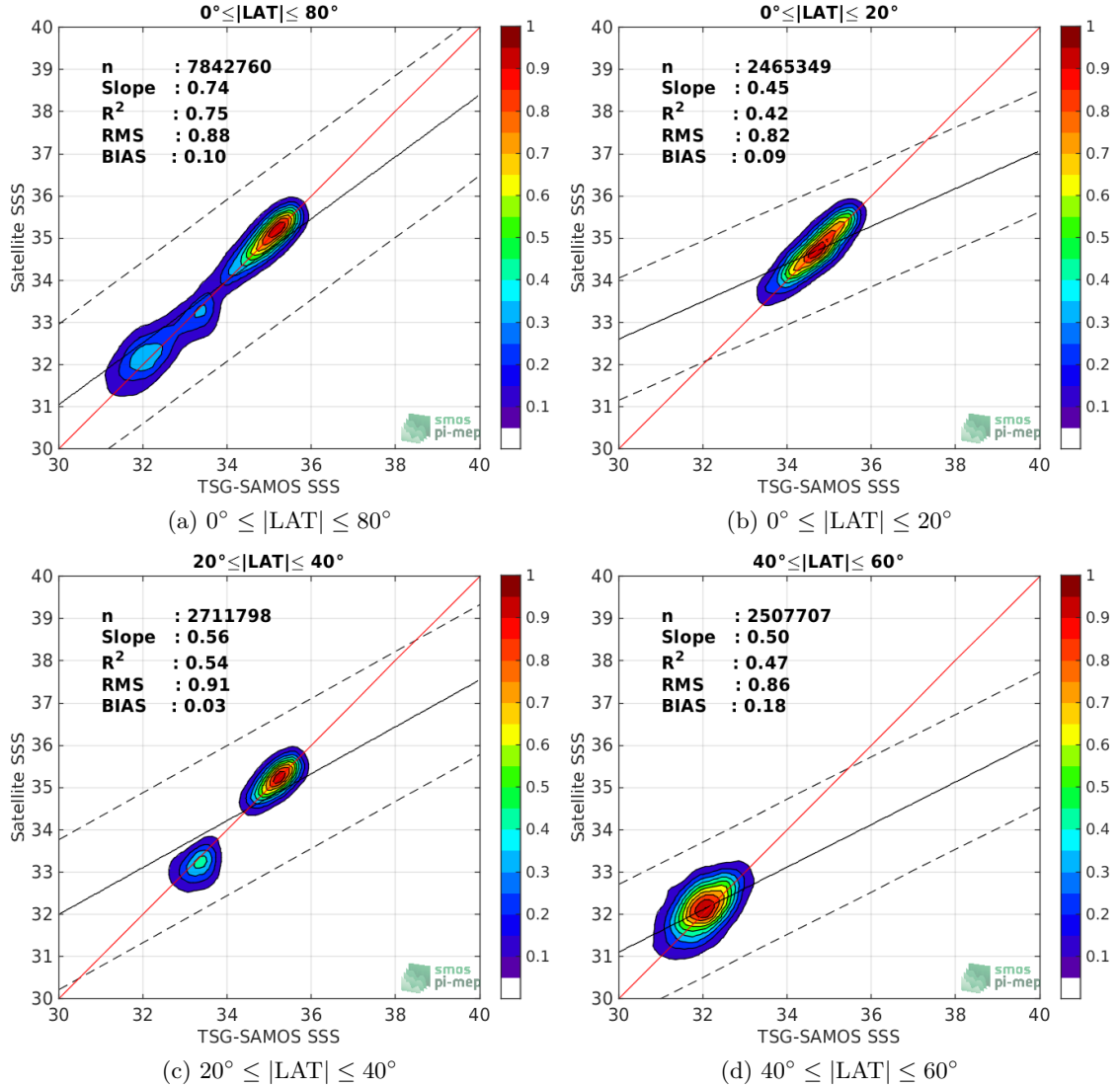
Figure 9: Contour maps of the concentration of SMOS-L3-CATDS-CECOS-LOCEAN-V4-18DAYS-25KM SSS (y-axis) versus TSG-SAMOS SSS (x-axis) at match-up pairs for different latitude bands. For each plot, the red line shows x=y . The black thin and dashed lines indicate a linear fit through the data cloud and the \pm 95\% confidence levels, respectively. The number match-up pairs n , the slope and R^2 coefficient of the linear fit, the root mean square (RMS) and the mean bias between satellite and in situ data are indicated for each latitude band in each plots.
