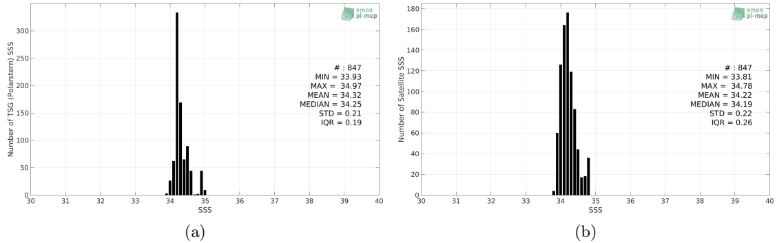
Figure 2: Histograms of SSS from TSG (Polarstern) (a) and SMOS SSS L3 v4 - 18 Days (CATDS-CECOS-LOCEAN) (b) considering all match-up pairs per bins of 0.1 over the Pacific Ocean Pi-MEP region and for the full satellite product period.
