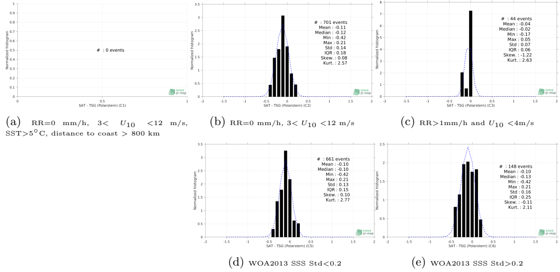
Figure 13: Normalized histogram of \Delta SSS (SMOS SSS L3 v4 - 18 Days (CATDS-CECOS-LOCEAN) - TSG (Polarstern)) for 5 different subdatasets corresponding to: RR=0 mm/h, 3 < U_{10} < 12 m/s, SST > 5^\circ C , distance to coast > 800 km (a), RR=0 mm/h, 3 < U_{10} < 12 m/s (b), RR > 1 mm/h and U_{10} < 4 m/s (c), WOA2013 SSS Std < 0.2 (d), WOA2013 SSS Std > 0.2 (e).
