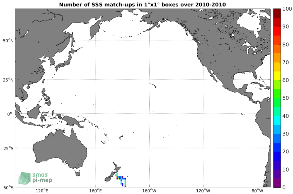
Figure 4: Number of SSS match-ups between TSG (Polarstern) SSS and the SMOS SSS L3 v4 - 18 Days (CATDS-CECOS-LOCEAN) SSS product for the Pacific Ocean Pi-MEP region over 1°x1° boxes and for the full satellite product period.
