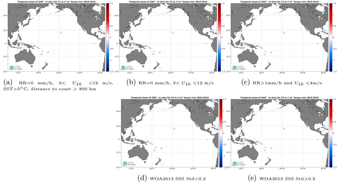
Figure 12: Temporal mean gridded over spatial boxes of size 1^{\circ}\times 1^{\circ} of \Delta\text{SSS} (SMOS SSS L3 v4 - 18 Days (CATDS-CECOS-LOCEAN) - TSG (Polarstern)) for 5 different subdatasets corresponding to:RR=0 mm/h, 3 < U_{10} < 12 m/s, SST >5^{\circ}\text{C} , distance to coast > 800 km (a), RR=0 mm/h, 3 < U_{10} < 12 m/s (b), RR >1 mm/h and U_{10} < 4 m/s (c), WOA2013 SSS Std <0.2 (d), WOA2013 SSS Std >0.2 (e).
