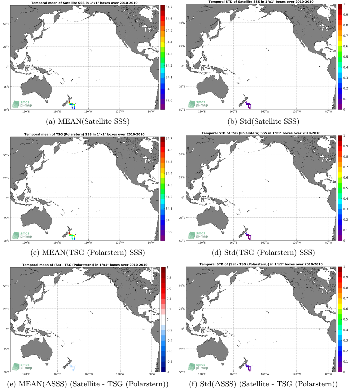
Figure 6: Temporal mean (left) and Std (right) of SSS from SMOS SSS L3 v4 - 18 Days (CATDS-CECOS-LOCEAN) (top), TSG (Polarstern) (middle), and of \Delta SSS (Satellite - TSG (Polarstern)). Only match-up pairs are used to generate these maps.
