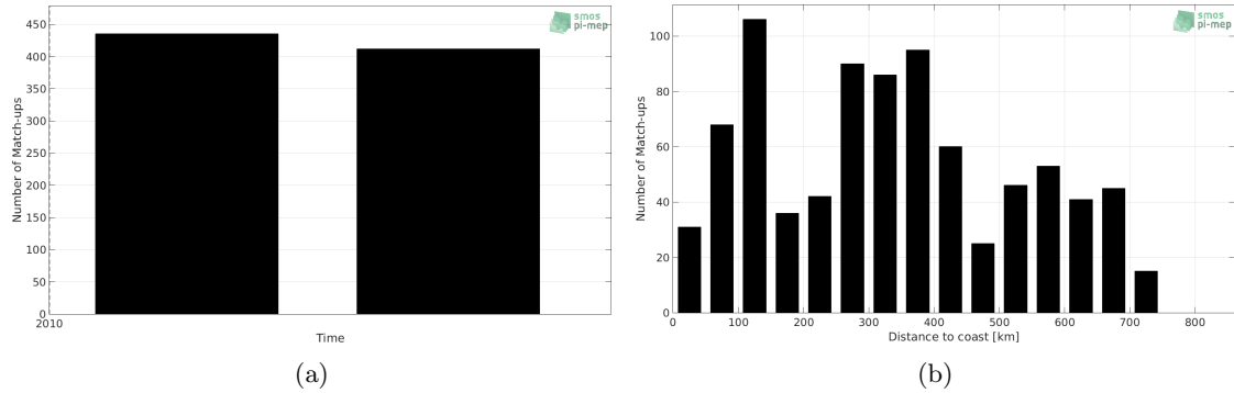
Figure 1: Number of match-ups between TSG (Polarstern) and SMOS SSS L3 v4 - 18 Days (CATDS-CECOS-LOCEAN) SSS as a function of time (a) and as function of the distance to coast (b) over the Pacific Ocean Pi-MEP region and for the full satellite product period.
