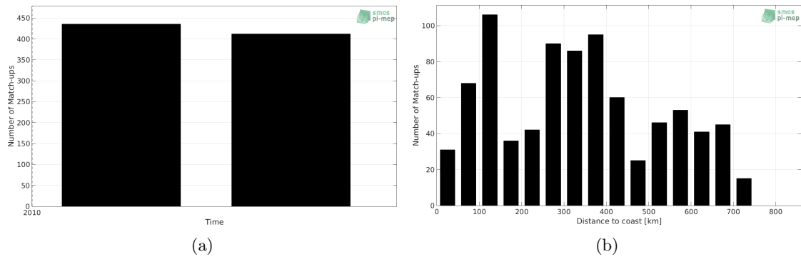
Figure 1: Number of match-ups between TSG-POLARSTERN and SMOS-L3-CATDS-CECOS-LOCEAN-V4-18DAYS-25KM SSS as a function of time (a) and as function of the distance to coast (b) over the Pacific Ocean Pi-MEP region and for the full satellite product period.
