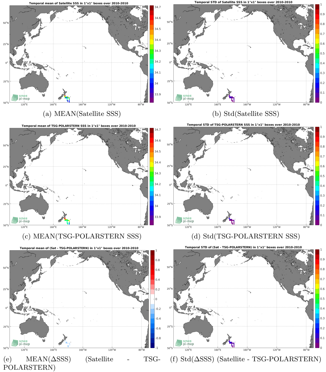
Figure 6: Temporal mean (left) and Std (right) of SSS from SMOS-L3-CATDS-CECOS-LOCEAN-V4-18DAYS-25KM (top), TSG-POLARSTERN (middle), and of \Delta SSS (Satellite - TSG-POLARSTERN). Only match-up pairs are used to generate these maps.
