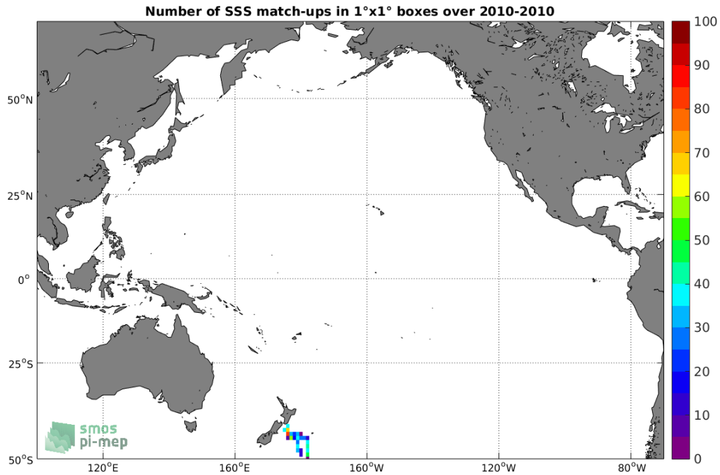
Figure 4: Number of SSS match-ups between TSG-POLARSTERN SSS and the SMOS-L3-CATDS-CECOS-LOCEAN-V4-18DAYS-25KM SSS product for the Pacific Ocean Pi-MEP region over 1°x1° boxes and for the full satellite product period.
