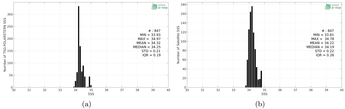
Figure 2: Histograms of SSS from TSG-POLARSTERN (a) and SMOS-L3-CATDS-CECOS-LOCEAN-V4-18DAYS-25KM (b) considering all match-up pairs per bins of 0.1 over the Pacific Ocean Pi-MEP region and for the full satellite product period.
