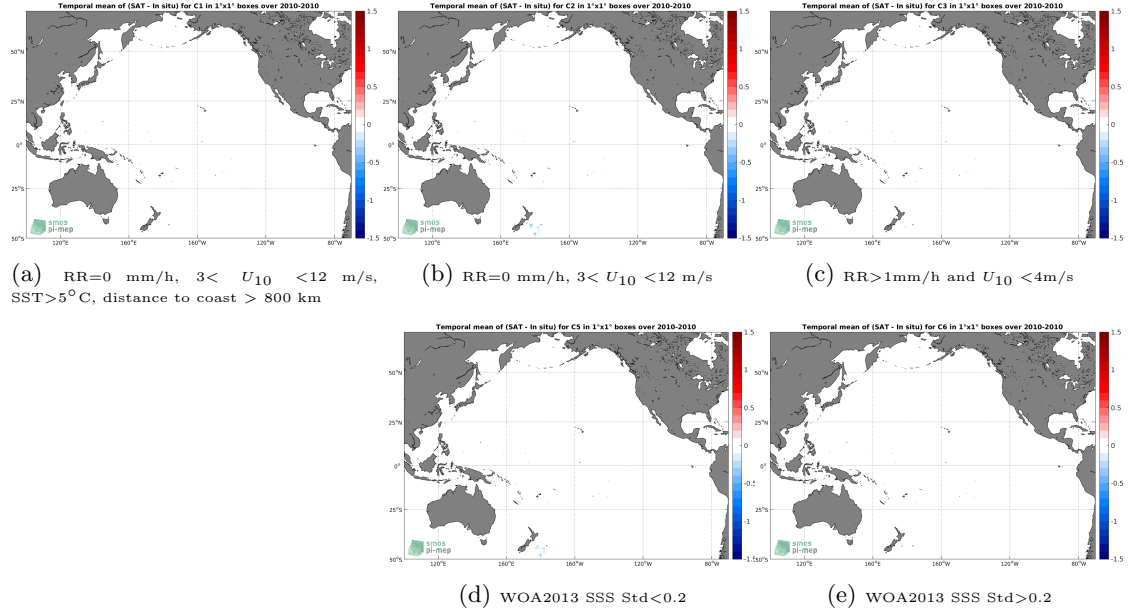
Figure 12: Temporal mean gridded over spatial boxes of size 1^{\circ}\times 1^{\circ} of \Delta\text{SSS} (SMOS-L3-CATDS-CECOS-LOCEAN-V4-18DAYS-25KM - TSG-POLARSTERN) for 5 different subdatasets corresponding to: RR=0 mm/h, 3 < U_{10} < 12 m/s, SST >5^{\circ}\text{C} , distance to coast > 800 km (a), RR=0 mm/h, 3 < U_{10} < 12 m/s (b), RR >1 mm/h and U_{10} < 4 m/s (c), WOA2013 SSS Std <0.2 (d), WOA2013 SSS Std >0.2 (e).
