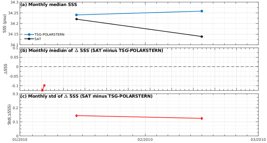
Figure 7: Time series of the monthly median SSS (top), median of \Delta\text{SSS} (Satellite - TSG-POLARSTERN) and Std of \Delta\text{SSS} (Satellite - TSG-POLARSTERN) over the Pacific Ocean Pi-MEP region considering all match-ups collected by the Pi-MEP.
