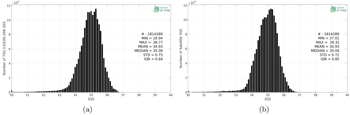
Figure 2: Histograms of SSS from TSG (LEGOS-DM) (a) and SMOS SSS L3 v4 - 18 Days (CATDS-CECOS-LOCEAN) (b) considering all match-up pairs per bins of 0.1 over the Pacific Ocean Pi-MEP region and for the full satellite product period.
