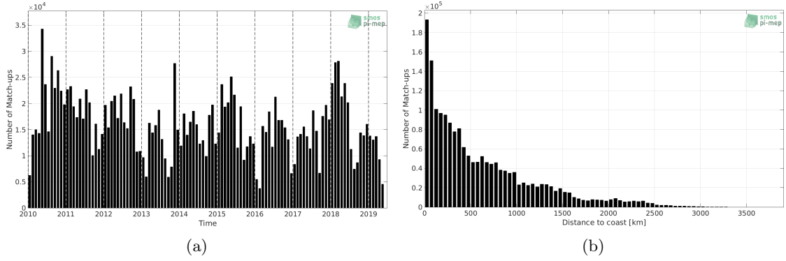
Figure 1: Number of match-ups between TSG (LEGOS-DM) and SMOS SSS L3 v4 - 18 Days (CATDS-CECOS-LOCEAN) SSS as a function of time (a) and as function of the distance to coast (b) over the Pacific Ocean Pi-MEP region and for the full satellite product period.
