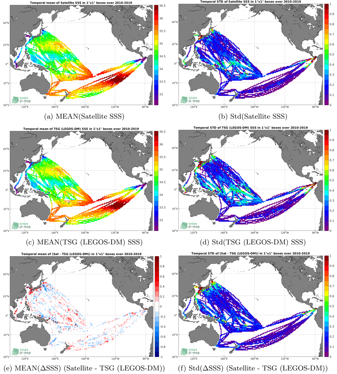
Figure 6: Temporal mean (left) and Std (right) of SSS from SMOS SSS L3 v4 - 18 Days (CATDS-CECOS-LOCEAN) (top), TSG (LEGOS-DM) (middle), and of \Delta SSS (Satellite - TSG (LEGOS-DM)). Only match-up pairs are used to generate these maps.
