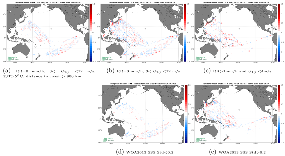
Figure 12: Temporal mean gridded over spatial boxes of size 1^\circ \times 1^\circ of \Delta SSS (SMOS SSS L3 v4 - 18 Days (CATDS-CECOS-LOCEAN) - TSG (LEGOS-DM)) for 5 different subdatasets corresponding to:RR=0 mm/h, 3 < U_{10} < 12 m/s, SST >5^\circ\text{C} , distance to coast > 800 km (a), RR=0 mm/h, 3 < U_{10} < 12 m/s (b), RR >1 mm/h and U_{10} < 4 m/s (c), WOA2013 SSS Std <0.2 (d), WOA2013 SSS Std >0.2 (e).
