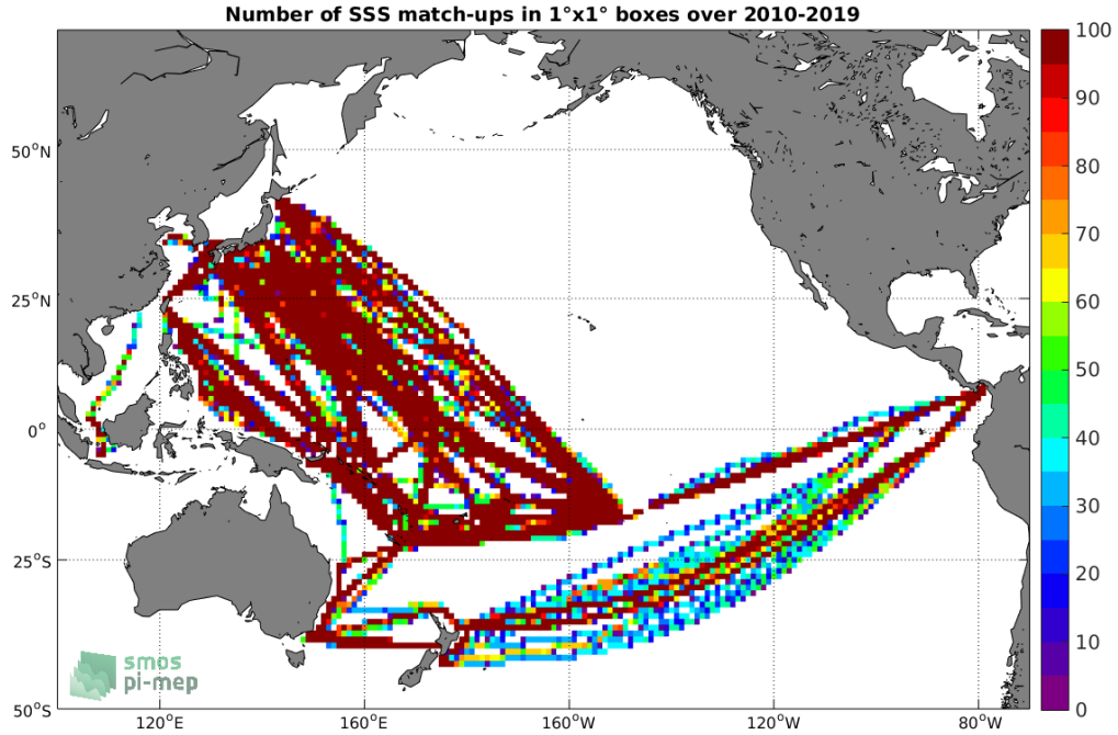
Figure 4: Number of SSS match-ups between TSG (LEGOS-DM) SSS and the SMOS SSS L3 v4 - 18 Days (CATDS-CECOS-LOCEAN) SSS product for the Pacific Ocean Pi-MEP region over 1°x1° boxes and for the full satellite product period.
