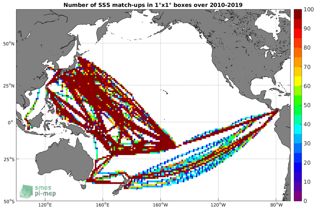
Figure 4: Number of SSS match-ups between TSG-LEGOS-DM SSS and the SMOS-L3-CATDS-CECOS-LOCEAN-V4-18DAYS-25KM SSS product for the Pacific Ocean Pi-MEP region over 1°x1° boxes and for the full satellite product period.
