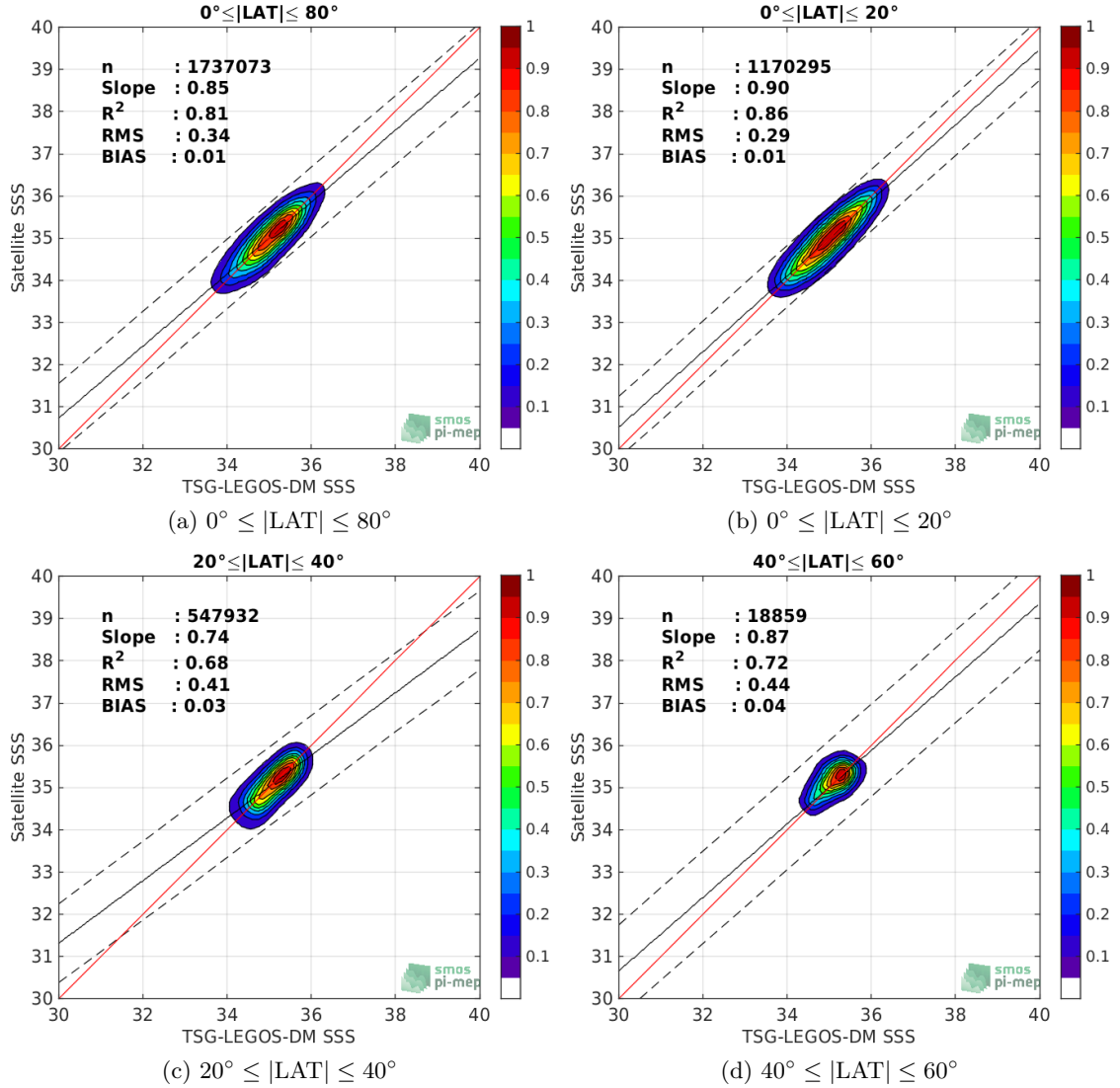
Figure 9: Contour maps of the concentration of SMOS-L3-CATDS-CECOS-LOCEAN-V4-18DAYS-25KM SSS (y-axis) versus TSG-LEGOS-DM SSS (x-axis) at match-up pairs for different latitude bands. For each plot, the red line shows x=y . The black thin and dashed lines indicate a linear fit through the data cloud and the \pm 95\% confidence levels, respectively. The number match-up pairs n , the slope and R^2 coefficient of the linear fit, the root mean square (RMS) and the mean bias between satellite and in situ data are indicated for each latitude band in each plots.
