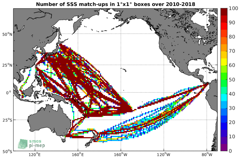
Figure 4: Number of SSS match-ups between TSG-LEGOS-DM SSS and the SMOS-L3-CATDS-CECOS-LOCEAN-V4-18DAYS-25KM SSS product for the Pacific Ocean Pi-MEP region over 1^\circ \times 1^\circ boxes and for the full satellite product period.
