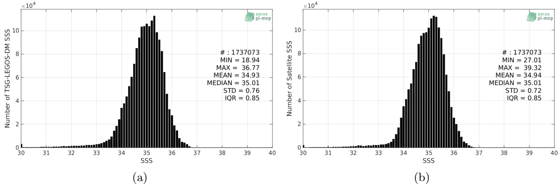
Figure 2: Histograms of SSS from TSG-LEGOS-DM (a) and SMOS-L3-CATDS-CECOS-LOCEAN-V4-18DAYS-25KM (b) considering all match-up pairs per bins of 0.1 over the Pacific Ocean Pi-MEP region and for the full satellite product period.
