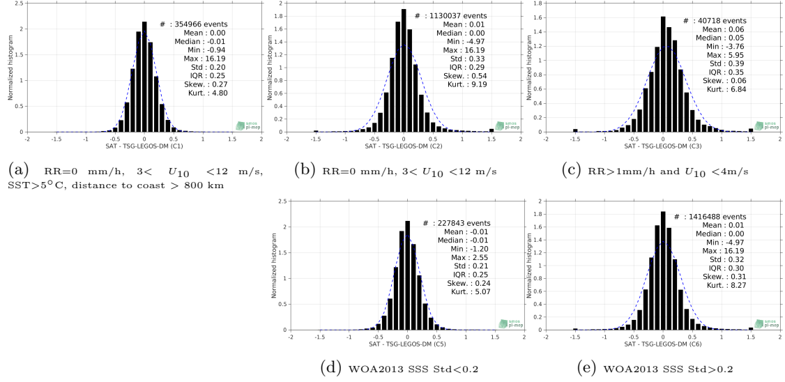
Figure 13: Normalized histogram of \Delta SSS (SMOS-L3-CATDS-CECOS-LOCEAN-V4-18DAYS-25KM - TSG-LEGOS-DM) for 5 different subdatasets corresponding to: RR=0 mm/h, 3 < U_{10} < 12 m/s, SST > 5^\circ\text{C} , distance to coast > 800 km (a), RR=0 mm/h, 3 < U_{10} < 12 m/s (b), RR > 1\text{mm/h} and U_{10} < 4\text{m/s} (c), WOA2013 SSS Std < 0.2 (d), WOA2013 SSS Std > 0.2 (e).
