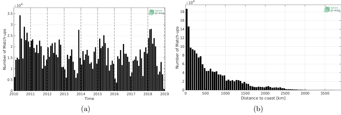
Figure 1: Number of match-ups between TSG-LEGOS-DM and SMOS-L3-CATDS-CECOS-LOCEAN-V4-18DAYS-25KM SSS as a function of time (a) and as function of the distance to coast (b) over the Pacific Ocean Pi-MEP region and for the full satellite product period.
