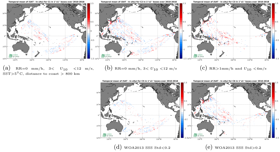
Figure 12: Temporal mean gridded over spatial boxes of size 1^\circ \times 1^\circ of \Delta SSS (SMOS-L3-CATDS-CECOS-LOCEAN-V4-18DAYS-25KM - TSG-LEGOS-DM) for 5 different subdatasets corresponding to: RR=0 mm/h, 3 < U_{10} < 12 m/s, SST >5^\circ C, distance to coast > 800 km (a), RR=0 mm/h, 3 < U_{10} < 12 m/s (b), RR >1 mm/h and U_{10} < 4 m/s (c), WOA2013 SSS Std <0.2 (d), WOA2013 SSS Std >0.2 (e).
