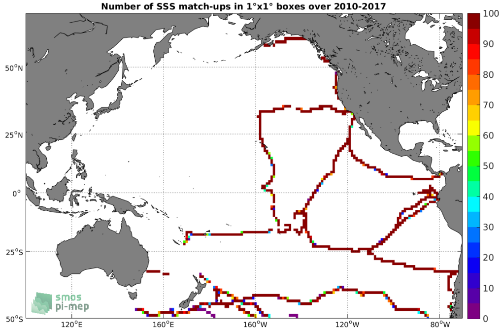
Figure 4: Number of SSS match-ups between TSG (GOSUD-Sailing-ship) SSS and the SMOS SSS L3 v4 - 18 Days (CATDS-CECOS-LOCEAN) SSS product for the Pacific Ocean Pi-MEP region over 1°x1° boxes and for the full satellite product period.
