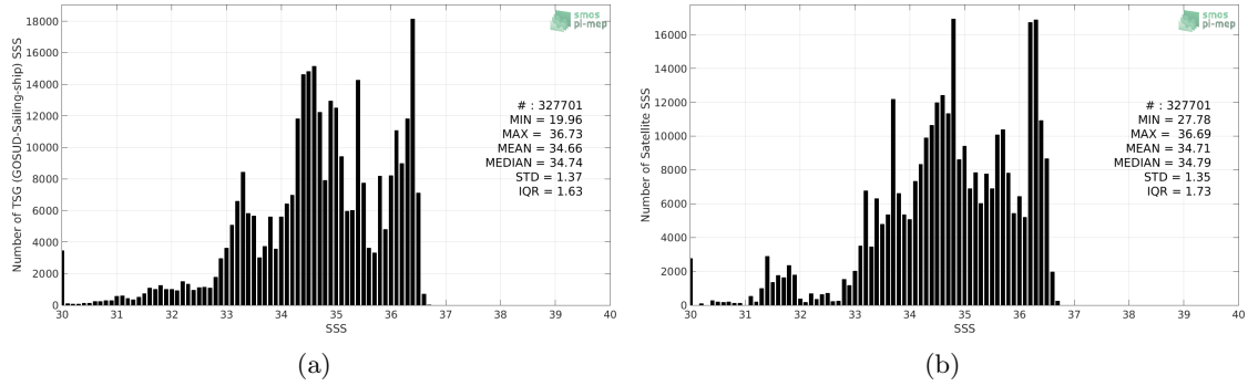
Figure 2: Histograms of SSS from TSG (GOSUD-Sailing-ship) (a) and SMOS SSS L3 v4 - 18 Days (CATDS-CECOS-LOCEAN) (b) considering all match-up pairs per bins of 0.1 over the Pacific Ocean Pi-MEP region and for the full satellite product period.
