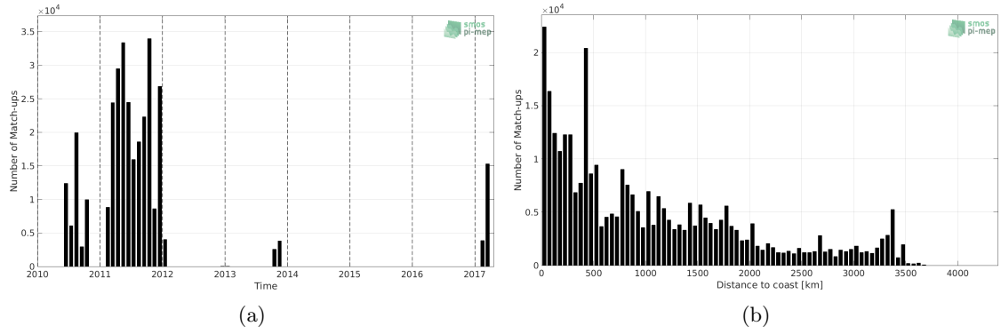
Figure 1: Number of match-ups between TSG (GOSUD-Sailing-ship) and SMOS SSS L3 v4 - 18 Days (CATDS-CECOS-LOCEAN) SSS as a function of time (a) and as function of the distance to coast (b) over the Pacific Ocean Pi-MEP region and for the full satellite product period.
