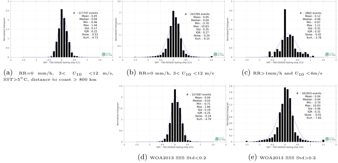
Figure 13: Normalized histogram of \Delta SSS (SMOS-L3-CATDS-CECOS-LOCEAN-V4-18DAYS-25KM - TSG-GOSUD-Sailing-ship) for 5 different subdatasets corresponding to: RR=0 mm/h, 3 < U_{10} < 12 m/s, SST>5°C, distance to coast > 800 km (a), RR=0 mm/h, 3 < U_{10} < 12 m/s (b), RR>1mm/h and U_{10} < 4 m/s (c), WOA2013 SSS Std<0.2 (d), WOA2013 SSS Std>0.2 (e).
