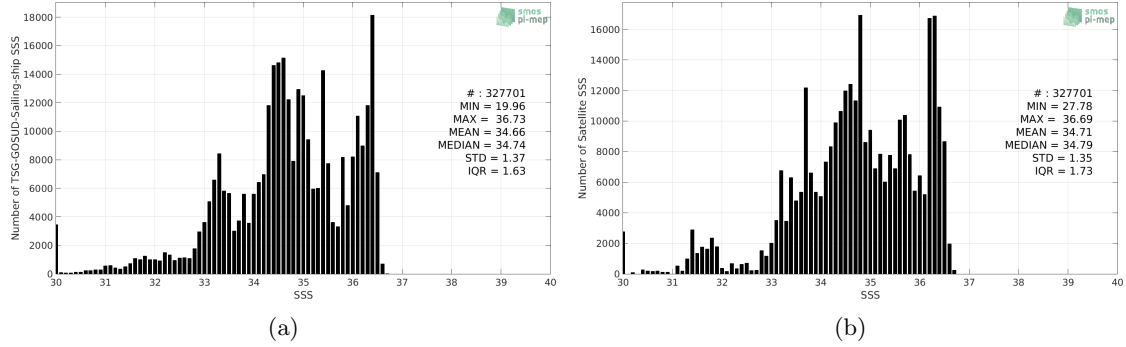
Figure 2: Histograms of SSS from TSG-GOSUD-Sailing-ship (a) and SMOS-L3-CATDS-CECOS-LOCEAN-V4-18DAYS-25KM (b) considering all match-up pairs per bins of 0.1 over the Pacific Ocean Pi-MEP region and for the full satellite product period.
