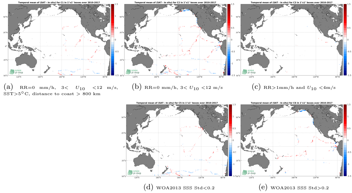
Figure 12: Temporal mean gridded over spatial boxes of size 1^\circ \times 1^\circ of \Delta SSS (SMOS-L3-CATDS-CECOS-LOCEAN-V4-18DAYS-25KM - TSG-GOSUD-Sailing-ship) for 5 different subdatasets corresponding to: RR=0 mm/h, 3 < U_{10} < 12 m/s, SST > 5^\circ\text{C} , distance to coast > 800 km (a), RR=0 mm/h, 3 < U_{10} < 12 m/s (b), RR > 1 mm/h and U_{10} < 4 m/s (c), WOA2013 SSS Std < 0.2 (d), WOA2013 SSS Std > 0.2 (e).
