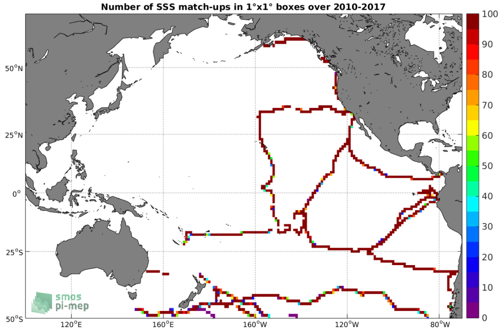
Figure 4: Number of SSS match-ups between TSG-GOSUD-Sailing-ship SSS and the SMOS-L3-CATDS-CECOS-LOCEAN-V4-18DAYS-25KM SSS product for the Pacific Ocean Pi-MEP region over 1°x1° boxes and for the full satellite product period.
