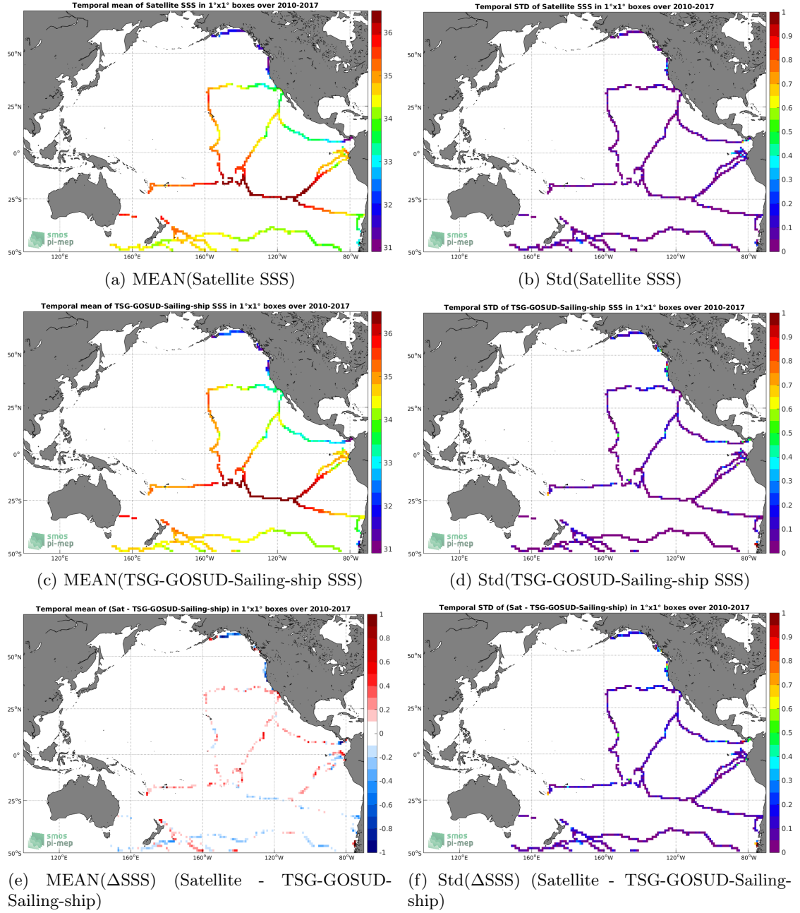
Figure 6: Temporal mean (left) and Std (right) of SSS from SMOS-L3-CATDS-CECOS-LOCEAN-V4-18DAYS-25KM (top), TSG-GOSUD-Sailing-ship (middle), and of \Delta SSS (Satellite - TSG-GOSUD-Sailing-ship). Only match-up pairs are used to generate these maps.
