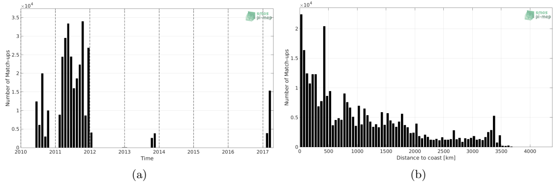
Figure 1: Number of match-ups between TSG-GOSUD-Sailing-ship and SMOS-L3-CATDS-CECOS-LOCEAN-V4-18DAYS-25KM SSS as a function of time (a) and as function of the distance to coast (b) over the Pacific Ocean Pi-MEP region and for the full satellite product period.
