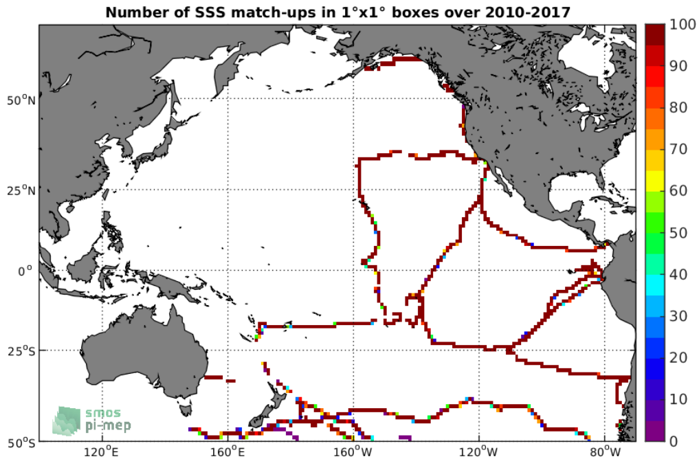
Figure 4: Number of SSS match-ups between TSG-GOSUD-Sailing-ship SSS and the SMOS-L3-CATDS-CECOS-LOCEAN-V4-18DAYS-25KM SSS product for the Pacific Ocean Pi-MEP region over 1^\circ \times 1^\circ boxes and for the full satellite product period.
