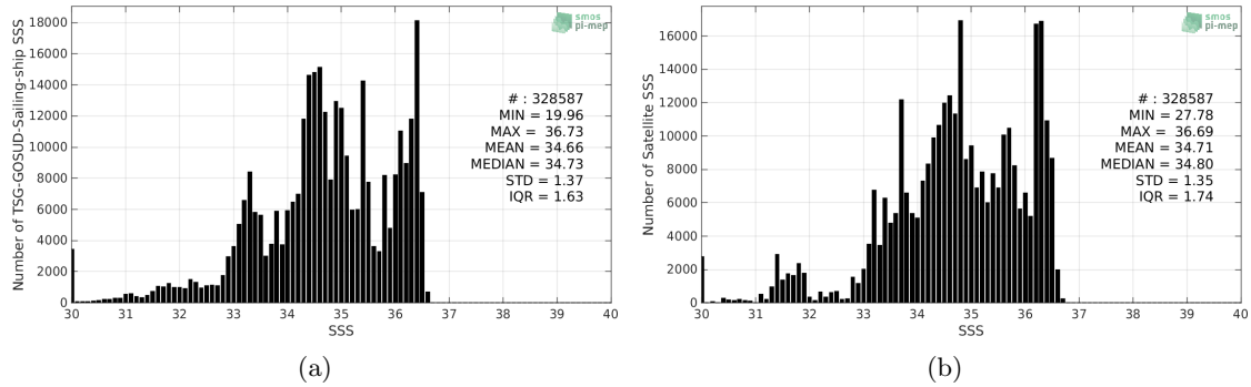
Figure 2: Histograms of SSS from TSG-GOSUD-Sailing-ship (a) and SMOS-L3-CATDS-CECOS-LOCEAN-V4-18DAYS-25KM (b) considering all match-up pairs per bins of 0.1 over the Pacific Ocean Pi-MEP region and for the full satellite product period.
