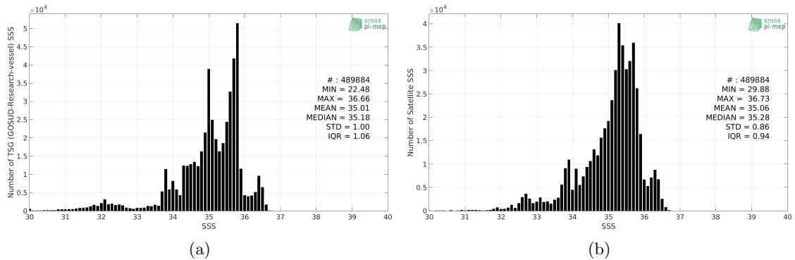
Figure 2: Histograms of SSS from TSG (GOSUD-Research-vessel) (a) and SMOS SSS L3 v4 - 18 Days (CATDS-CECOS-LOCEAN) (b) considering all match-up pairs per bins of 0.1 over the Pacific Ocean Pi-MEP region and for the full satellite product period.
