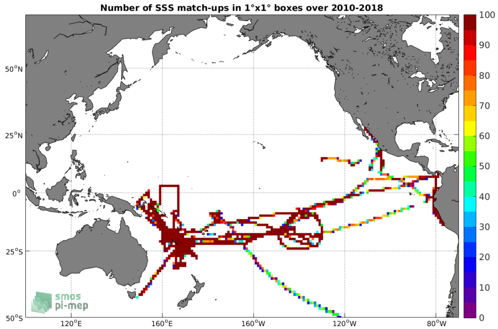
Figure 4: Number of SSS match-ups between TSG (GOSUD-Research-vessel) SSS and the SMOS SSS L3 v4 - 18 Days (CATDS-CECOS-LOCEAN) SSS product for the Pacific Ocean Pi-MEP region over 1°x1° boxes and for the full satellite product period.
