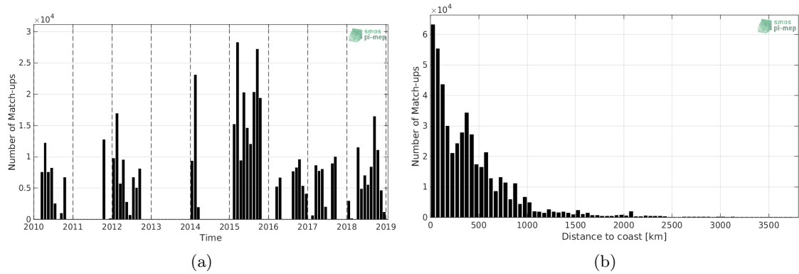
Figure 1: Number of match-ups between TSG-GOSUD-Research-vessel and SMOS-L3-CATDS-CECOS-LOCEAN-V4-18DAYS-25KM SSS as a function of time (a) and as function of the distance to coast (b) over the Pacific Ocean Pi-MEP region and for the full satellite product period.
