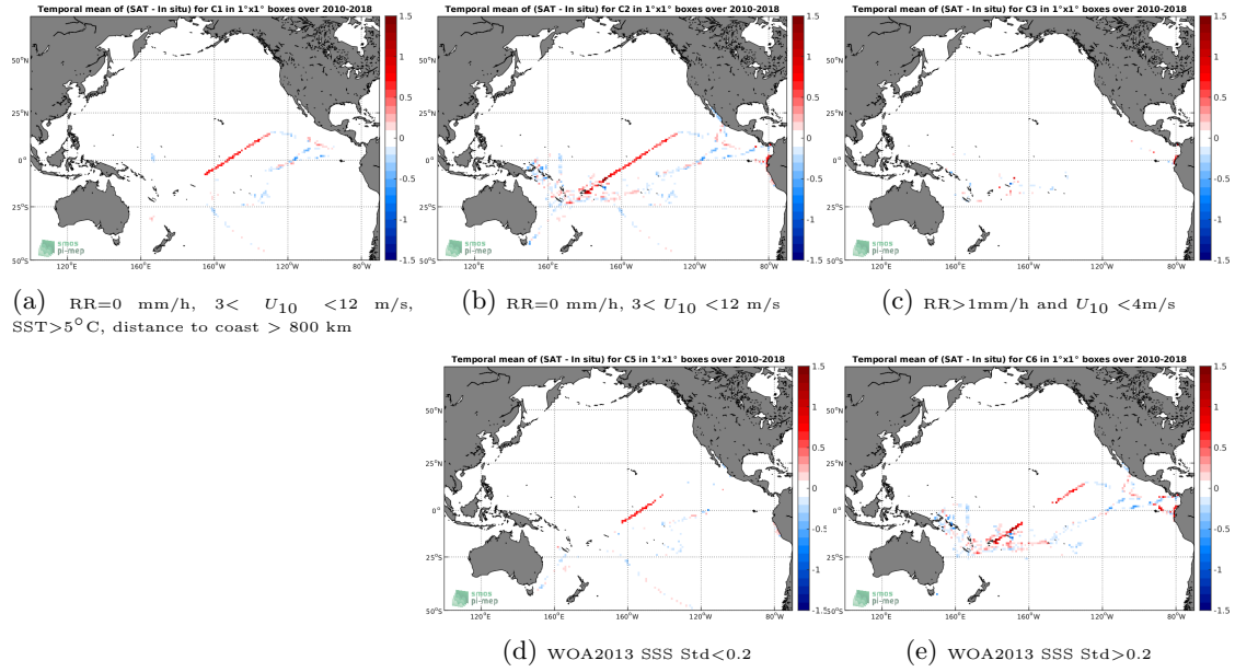
Figure 12: Temporal mean gridded over spatial boxes of size 1^\circ \times 1^\circ of \Delta SSS (SMOS-L3-CATDS-CECOS-LOCEAN-V4-18DAYS-25KM - TSG-GOSUD-Research-vessel) for 5 different subdatasets corresponding to: RR=0 mm/h, 3 < U_{10} < 12 m/s, SST >5^\circ C, distance to coast > 800 km (a), RR=0 mm/h, 3 < U_{10} < 12 m/s (b), RR >1 mm/h and U_{10} < 4 m/s (c), WOA2013 SSS Std <0.2 (d), WOA2013 SSS Std >0.2 (e).
