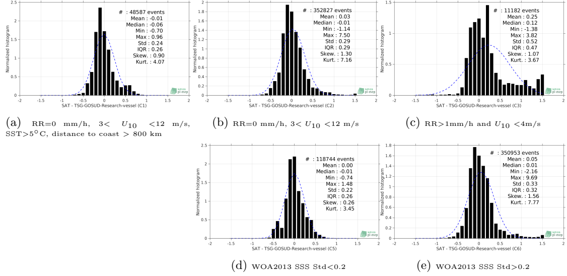
Figure 13: Normalized histogram of \Delta SSS (SMOS-L3-CATDS-CECOS-LOCEAN-V4-18DAYS-25KM - TSG-GOSUD-Research-vessel) for 5 different subdatasets corresponding to: RR=0 mm/h, 3 < U_{10} < 12 m/s, SST>5°C, distance to coast > 800 km (a), RR=0 mm/h, 3 < U_{10} < 12 m/s (b), RR>1mm/h and U_{10} < 4 m/s (c), WOA2013 SSS Std<0.2 (d), WOA2013 SSS Std>0.2 (e).
