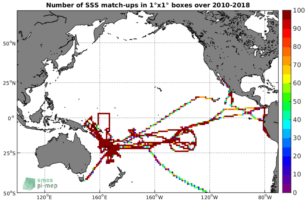
Figure 4: Number of SSS match-ups between TSG-GOSUD-Research-vessel SSS and the SMOS-L3-CATDS-CECOS-LOCEAN-V4-18DAYS-25KM SSS product for the Pacific Ocean Pi-MEP region over 1°x1° boxes and for the full satellite product period.
