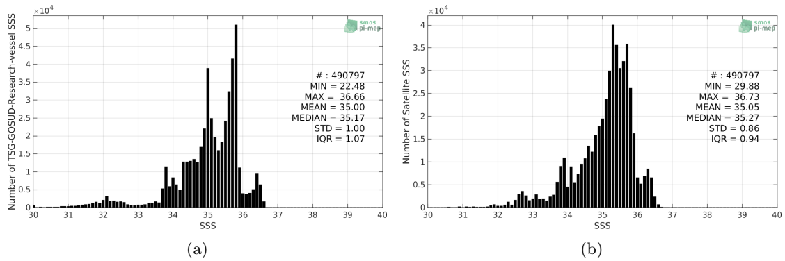
Figure 2: Histograms of SSS from TSG-GOSUD-Research-vessel (a) and SMOS-L3-CATDS-CECOS-LOCEAN-V4-18DAYS-25KM (b) considering all match-up pairs per bins of 0.1 over the Pacific Ocean Pi-MEP region and for the full satellite product period.
