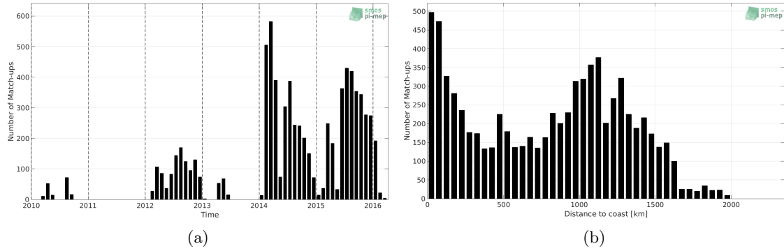
Figure 1: Number of match-ups between Sea mammals and SMOS SSS L3 v4 - 18 Days (CATDS-CECOS-LOCEAN) SSS as a function of time (a) and as function of the distance to coast (b) over the Pacific Ocean Pi-MEP region and for the full satellite product period.
