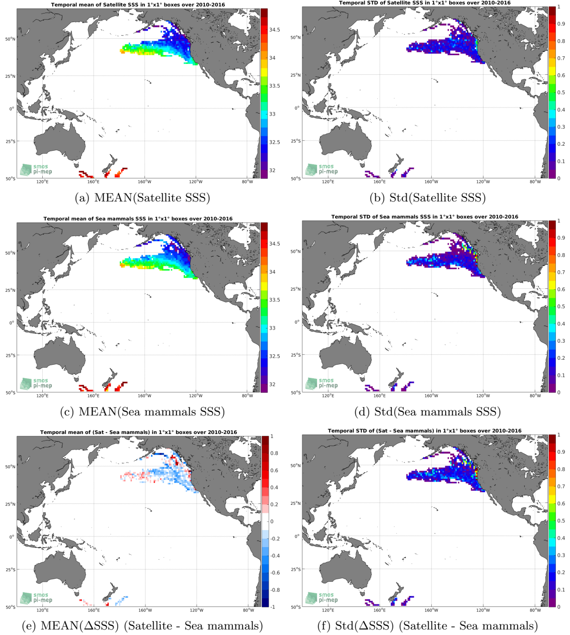
Figure 6: Temporal mean (left) and Std (right) of SSS from SMOS SSS L3 v4 - 18 Days (CATDS-CECOS-LOCEAN) (top), Sea mammals (middle), and of \Delta SSS (Satellite - Sea mammals). Only match-up pairs are used to generate these maps.
