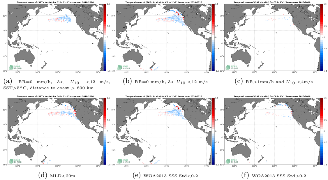
Figure 12: Temporal mean gridded over spatial boxes of size 1^\circ \times 1^\circ of \Delta SSS (SMOS SSS L3 v4 - 18 Days (CATDS-CECOS-LOCEAN) - Sea mammals) for 6 different subdatasets corresponding to: RR=0 mm/h, 3 < U_{10} < 12 m/s, SST >5^\circ\text{C} , distance to coast > 800 km (a), RR=0 mm/h, 3 < U_{10} < 12 m/s (b), RR >1 mm/h and U_{10} < 4 m/s (c),MLD <20 m (d),WOA2013 SSS Std <0.2 (e),WOA2013 SSS Std >0.2 (f).
