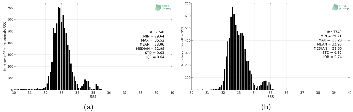
Figure 2: Histograms of SSS from Sea mammals (a) and SMOS SSS L3 v4 - 18 Days (CATDS-CECOS-LOCEAN) (b) considering all match-up pairs per bins of 0.1 over the Pacific Ocean Pi-MEP region and for the full satellite product period.
