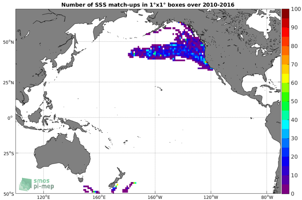
Figure 4: Number of SSS match-ups between Sea mammals SSS and the SMOS SSS L3 v4 - 18 Days (CATDS-CECOS-LOCEAN) SSS product for the Pacific Ocean Pi-MEP region over 1°x1° boxes and for the full satellite product period.
