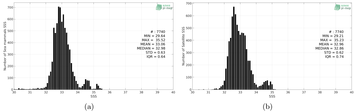
Figure 2: Histograms of SSS from Sea mammals (a) and SMOS-L3-CATDS-CECOS-LOCEAN-V4-18DAYS-25KM (b) considering all match-up pairs per bins of 0.1 over the Pacific Ocean Pi-MEP region and for the full satellite product period.
