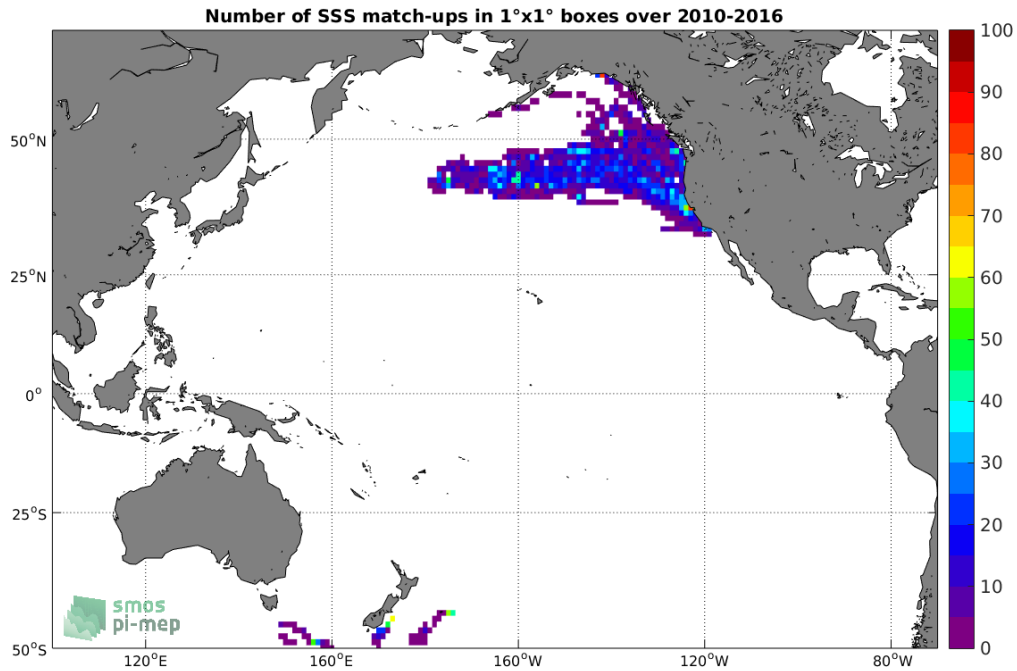
Figure 4: Number of SSS match-ups between Sea mammals SSS and the SMOS-L3-CATDS-CECOS-LOCEAN-V4-18DAYS-25KM SSS product for the Pacific Ocean Pi-MEP region over 1°x1° boxes and for the full satellite product period.
