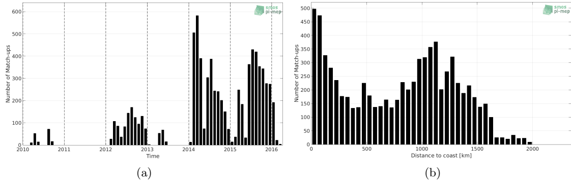
Figure 1: Number of match-ups between Sea mammals and SMOS-L3-CATDS-CECOS-LOCEAN-V4-18DAYS-25KM SSS as a function of time (a) and as function of the distance to coast (b) over the Pacific Ocean Pi-MEP region and for the full satellite product period.
