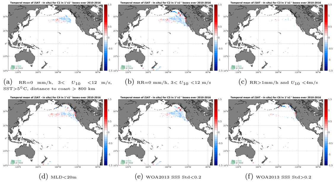
Figure 12: Temporal mean gridded over spatial boxes of size 1^\circ \times 1^\circ of \Delta SSS (SMOS-L3-CATDS-CECOS-LOCEAN-V4-18DAYS-25KM - Sea mammals) for 6 different subdatasets corresponding to: RR=0 mm/h, 3 < U_{10} < 12 m/s, SST >5^\circ C, distance to coast > 800 km (a), RR=0 mm/h, 3 < U_{10} < 12 m/s (b), RR >1 mm/h and U_{10} < 4 m/s (c),MLD <20 m (d),WOA2013 SSS Std <0.2 (e),WOA2013 SSS Std >0.2 (f).
