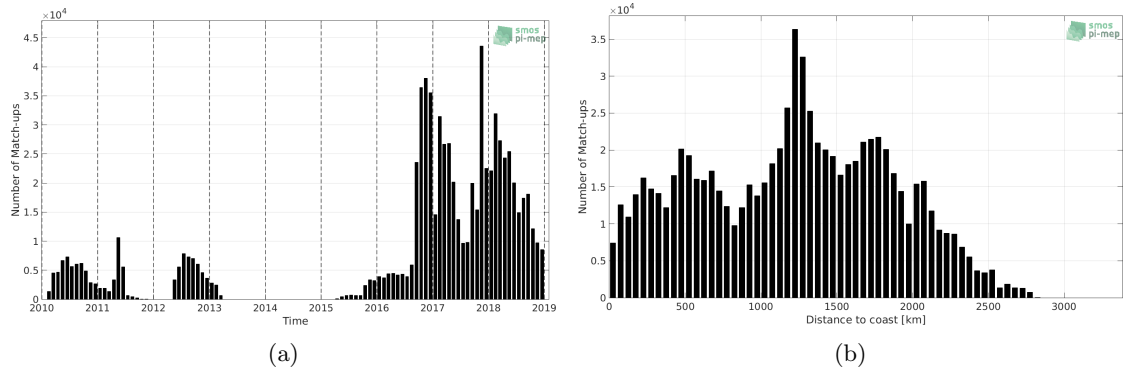
Figure 1: Number of match-ups between Surface drifters and SMOS SSS L3 v4 - 18 Days (CATDS-CECOS-LOCEAN) SSS as a function of time (a) and as function of the distance to coast (b) over the Pacific Ocean Pi-MEP region and for the full satellite product period.
