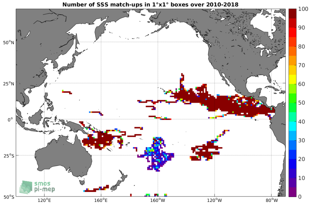
Figure 3: Number of SSS match-ups between Surface drifters SSS and the SMOS SSS L3 v4 - 18 Days (CATDS-CECOS-LOCEAN) SSS product for the Pacific Ocean Pi-MEP region over 1^\circ \times 1^\circ boxes and for the full satellite product period.
