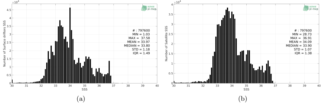
Figure 2: Histograms of SSS from Surface drifters (a) and SMOS SSS L3 v4 - 18 Days (CATDS-CECOS-LOCEAN) (b) considering all match-up pairs per bins of 0.1 over the Pacific Ocean Pi-MEP region and for the full satellite product period.
