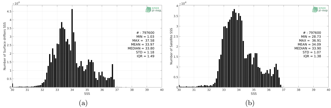
Figure 2: Histograms of SSS from Surface drifters (a) and SMOS-L3-CATDS-CECOS-LOCEAN-V4-18DAYS-25KM (b) considering all match-up pairs per bins of 0.1 over the Pacific Ocean Pi-MEP region and for the full satellite product period.
