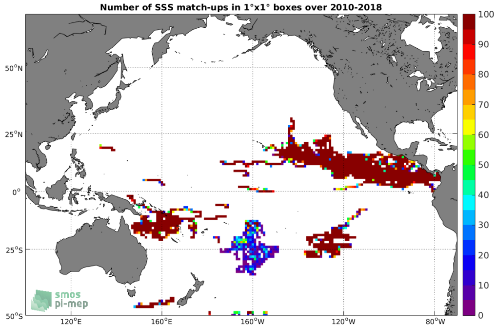
Figure 3: Number of SSS match-ups between Surface drifters SSS and the SMOS-L3-CATDS-CECOS-LOCEAN-V4-18DAYS-25KM SSS product for the Pacific Ocean Pi-MEP region over 1°x1° boxes and for the full satellite product period.
