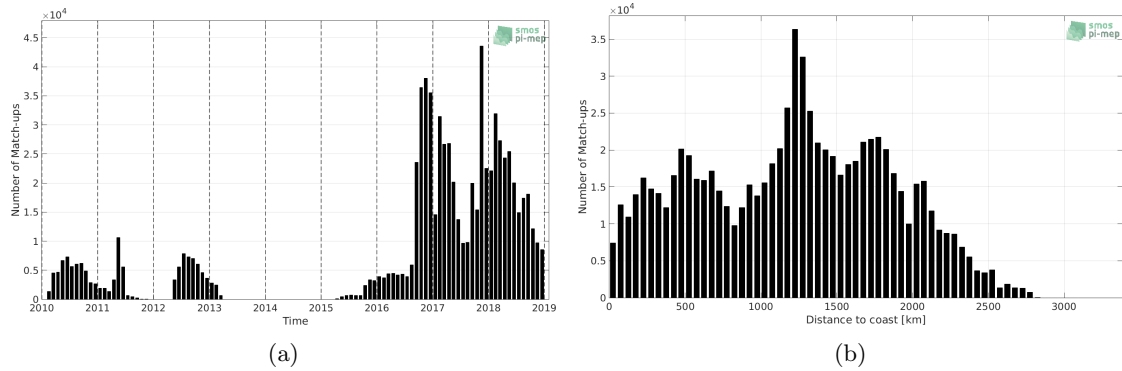
Figure 1: Number of match-ups between Surface drifters and SMOS-L3-CATDS-CECOS-LOCEAN-V4-18DAYS-25KM SSS as a function of time (a) and as function of the distance to coast (b) over the Pacific Ocean Pi-MEP region and for the full satellite product period.
