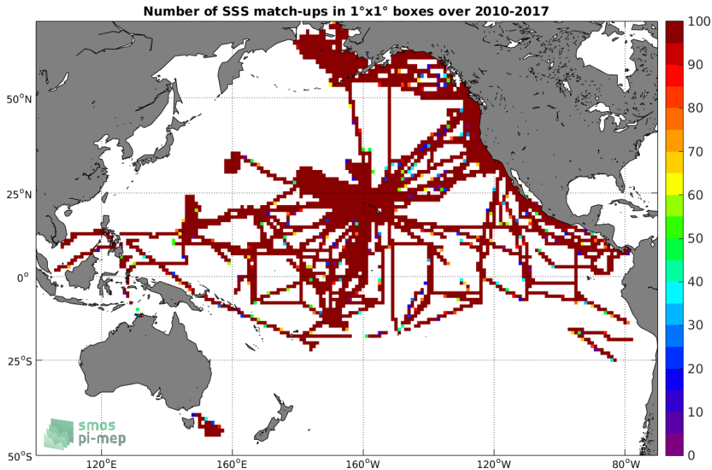
Figure 4: Number of SSS match-ups between TSG-SAMOS SSS and the SMOS-L3-CATDS-CECOS-LOCEAN-V3-9DAYS-25KM SSS product for the Pacific Ocean Pi-MEP region over 1^\circ \times 1^\circ boxes and for the full satellite product period.
