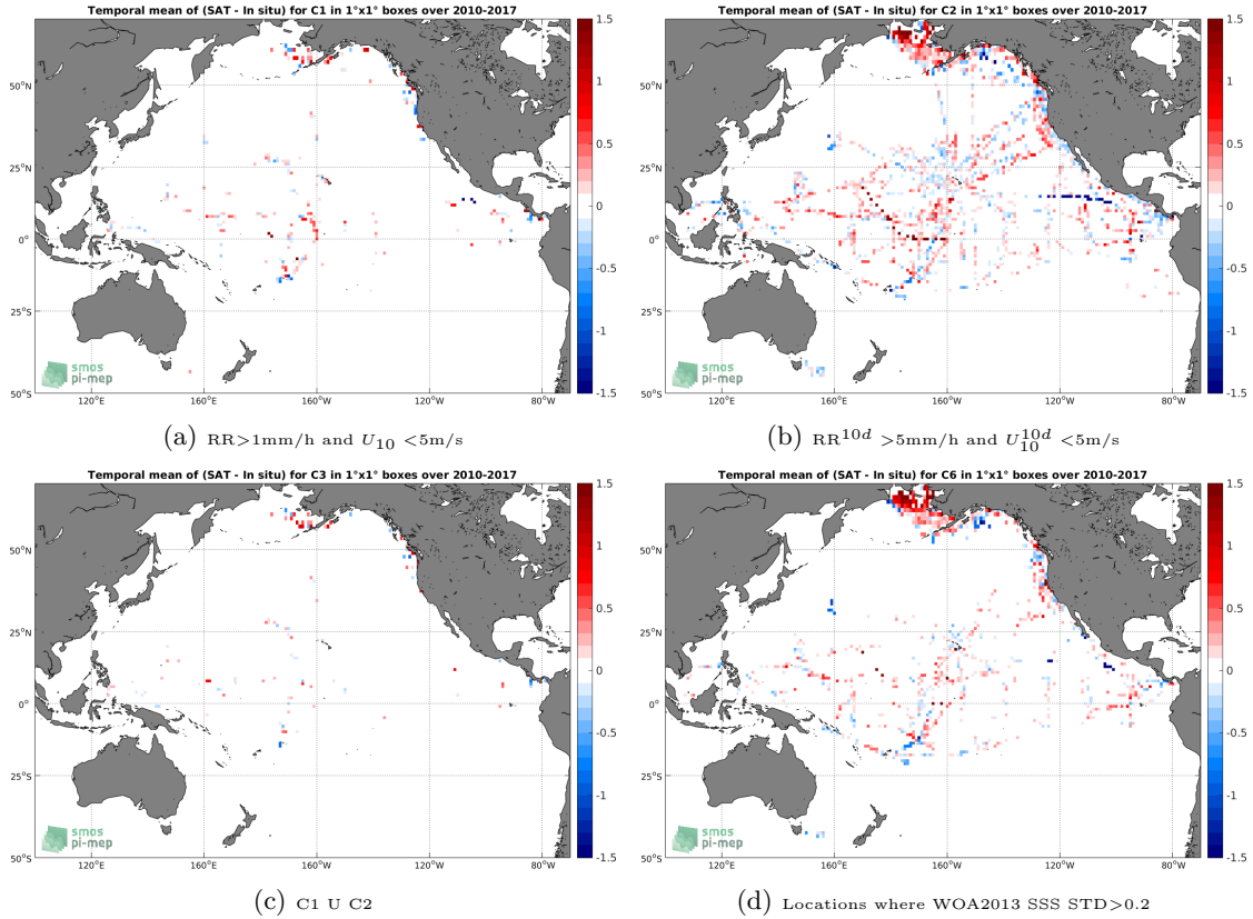
Figure 12: Temporal mean gridded over spatial boxes of size 1^\circ \times 1^\circ of \Delta SSS (SMOS-L3-CATDS-CECOS-LOCEAN-V3-9DAYS-25KM - TSG-SAMOS) for 4 different subdatasets corresponding to: RR > 1\text{mm/h} and U_{10} < 5\text{m/s} (a), RR^{10d} > 5\text{mm/h} and U_{10}^{10d} < 5\text{m/s} (b), C1 U C2 (c), Locations where WOA2013 SSS STD > 0.2 (d).
