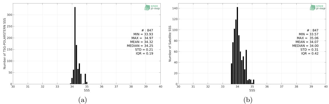
Figure 2: Histograms of SSS from TSG-POLARSTERN (a) and SMOS-L3-CATDS-CECOS-LOCEAN-V3-9DAYS-25KM (b) considering all match-up pairs per bins of 0.1 over the Pacific Ocean Pi-MEP region and for the full satellite product period.
