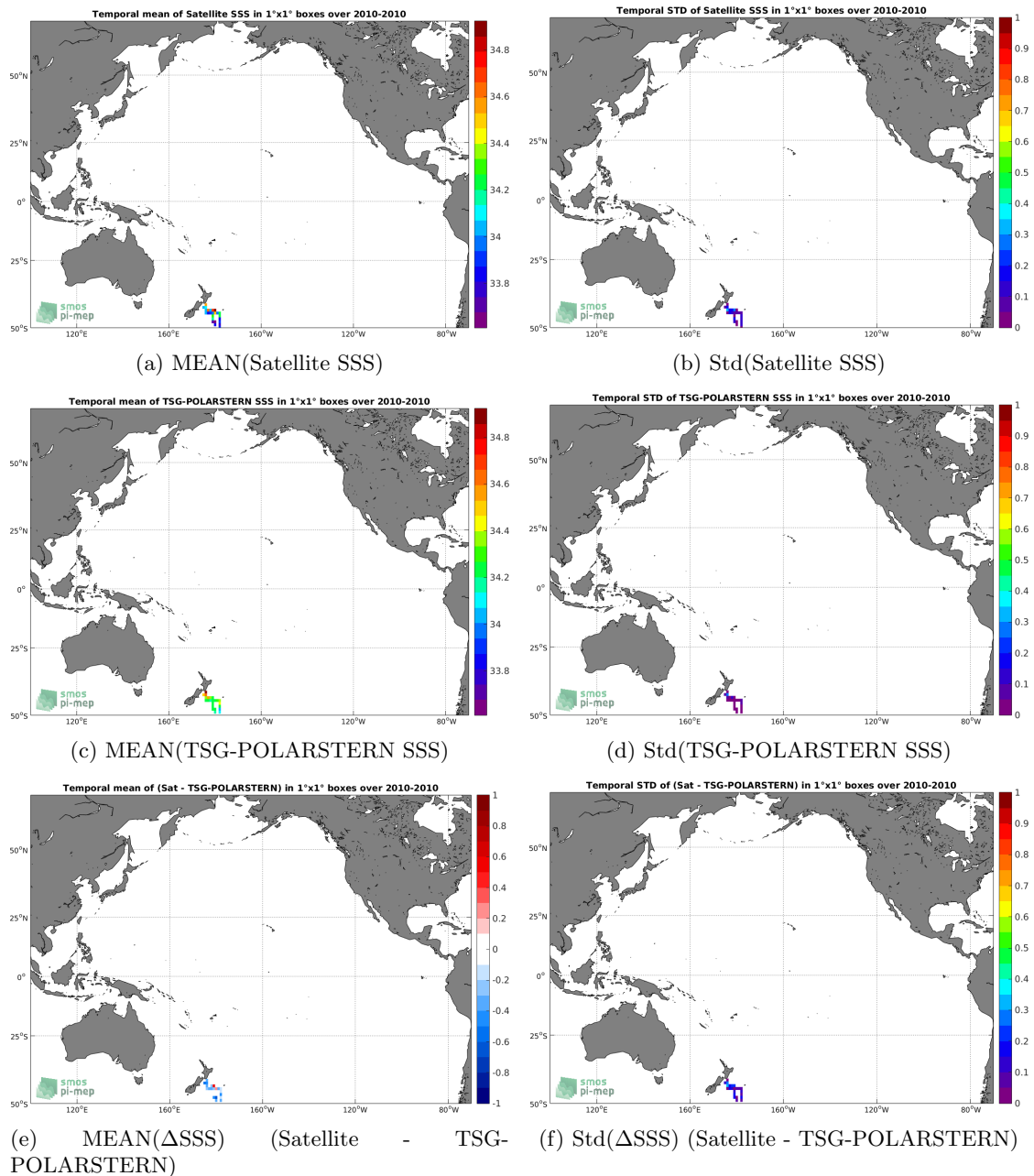
Figure 6: Temporal mean (left) and Std (right) of SSS from SMOS-L3-CATDS-CECOS-LOCEAN-V3-9DAYS-25KM (top), TSG-POLARSTERN (middle), and of \Delta SSS (Satellite - TSG-POLARSTERN). Only match-up pairs are used to generate these maps.
