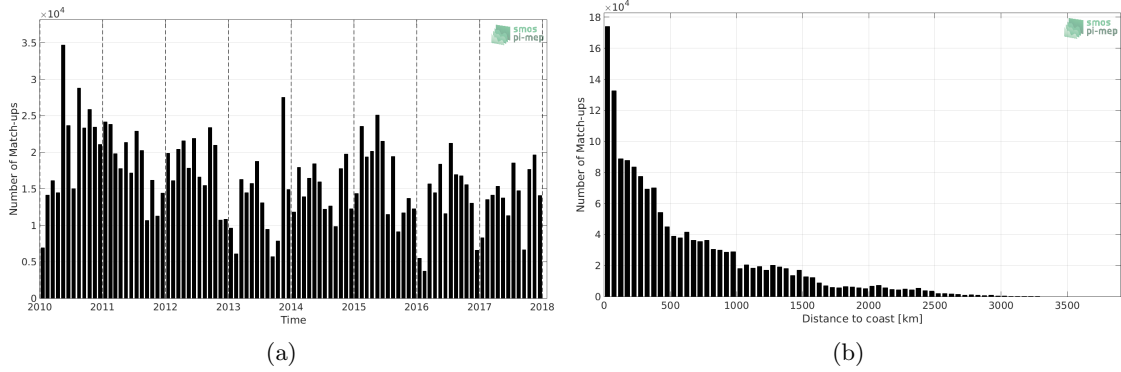
Figure 1: Number of match-ups between TSG-LEGOS-DM and SMOS-L3-CATDS-CECOS-LOCEAN-V3-9DAYS-25KM SSS as a function of time (a) and as function of the distance to coast (b) over the Pacific Ocean Pi-MEP region and for the full satellite product period.
