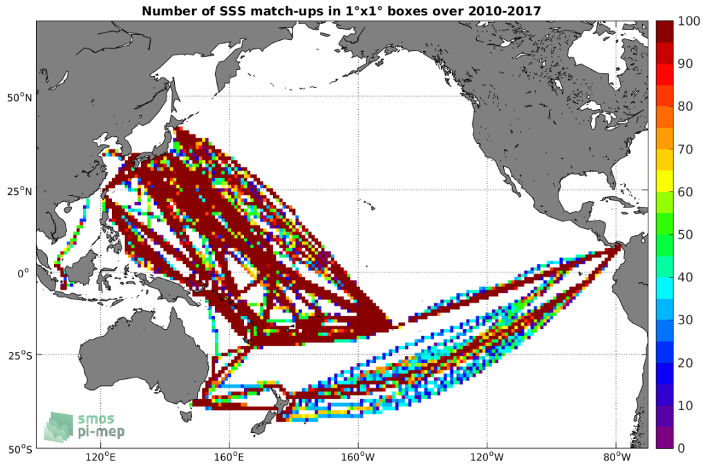
Figure 4: Number of SSS match-ups between TSG-LEGOS-DM SSS and the SMOS-L3-CATDS-CECOS-LOCEAN-V3-9DAYS-25KM SSS product for the Pacific Ocean Pi-MEP region over 1^\circ \times 1^\circ boxes and for the full satellite product period.
