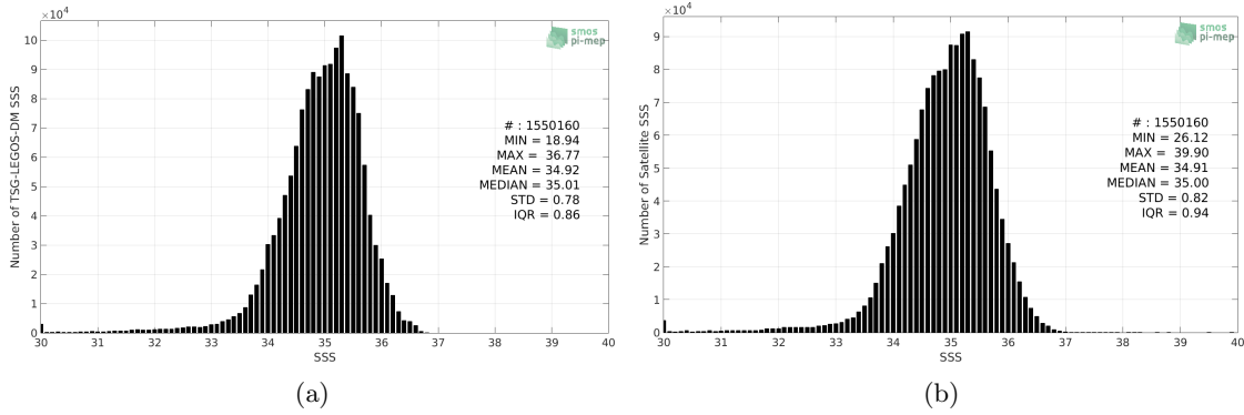
Figure 2: Histograms of SSS from TSG-LEGOS-DM (a) and SMOS-L3-CATDS-CECOS-LOCEAN-V3-9DAYS-25KM (b) considering all match-up pairs per bins of 0.1 over the Pacific Ocean Pi-MEP region and for the full satellite product period.
