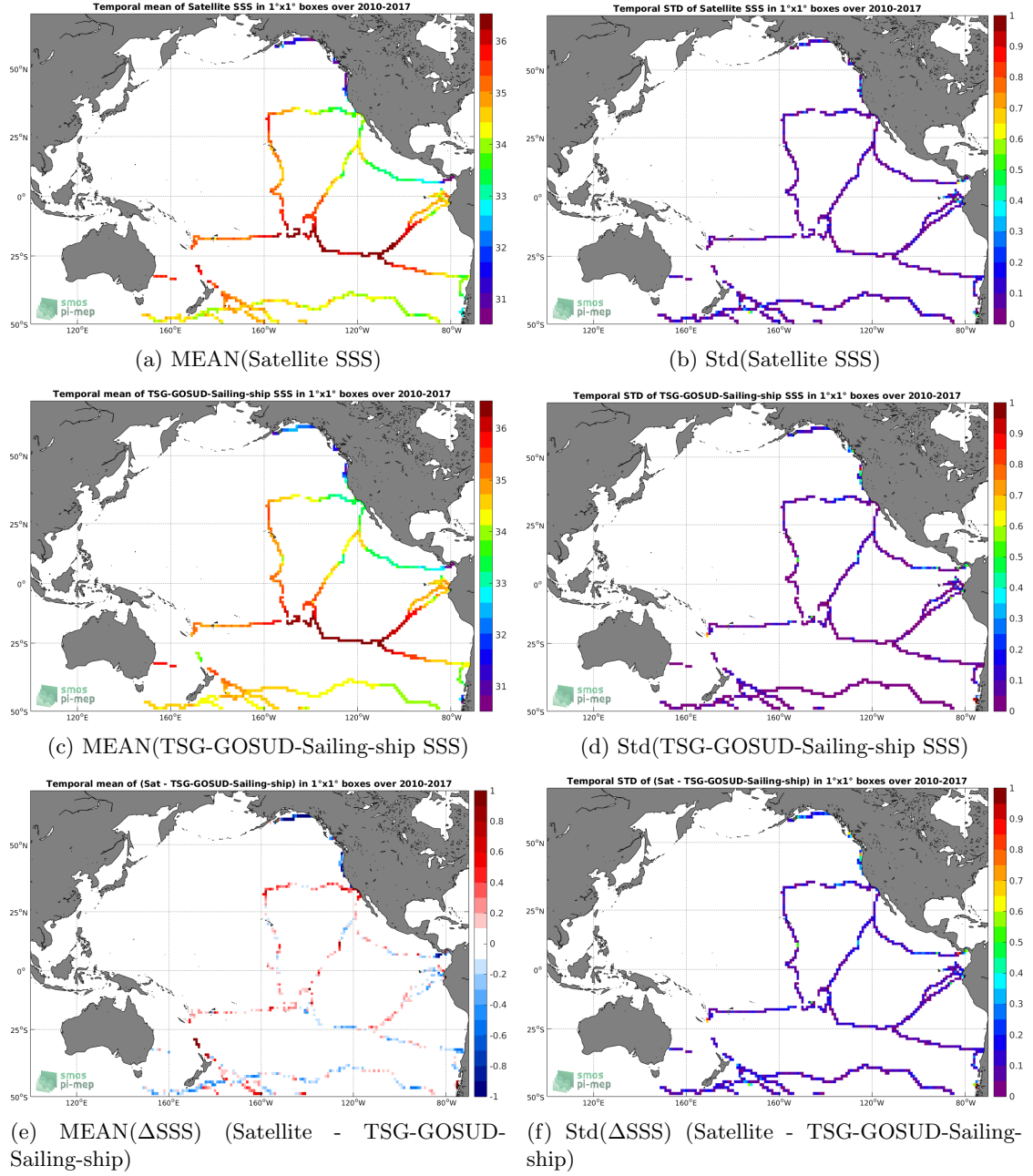
Figure 6: Temporal mean (left) and Std (right) of SSS from SMOS-L3-CATDS-CECOS-LOCEAN-V3-9DAYS-25KM (top), TSG-GOSUD-Sailing-ship (middle), and of \Delta SSS (Satellite - TSG-GOSUD-Sailing-ship). Only match-up pairs are used to generate these maps.
