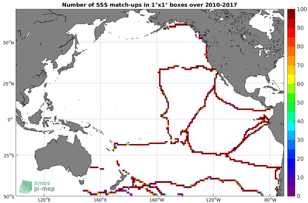
Figure 4: Number of SSS match-ups between TSG-GOSUD-Sailing-ship SSS and the SMOS-L3-CATDS-CECOS-LOCEAN-V3-9DAYS-25KM SSS product for the Pacific Ocean Pi-MEP region over 1^\circ \times 1^\circ boxes and for the full satellite product period.
