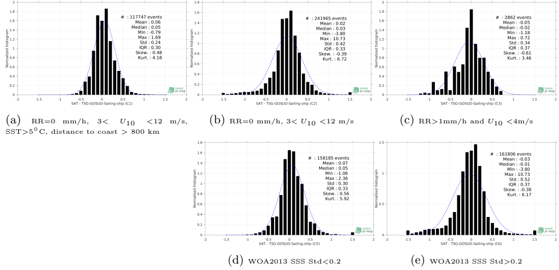
Figure 13: Normalized histogram of \Delta SSS (SMOS-L3-CATDS-CECOS-LOCEAN-V3-9DAYS-25KM - TSG-GOSUD-Sailing-ship) for 5 different subdatasets corresponding to: RR=0 mm/h, 3 < U_{10} < 12 m/s, SST>5°C, distance to coast > 800 km (a), RR=0 mm/h, 3 < U_{10} < 12 m/s (b), RR>1mm/h and U_{10} < 4 m/s (c), WOA2013 SSS Std<0.2 (d), WOA2013 SSS Std>0.2 (e).
