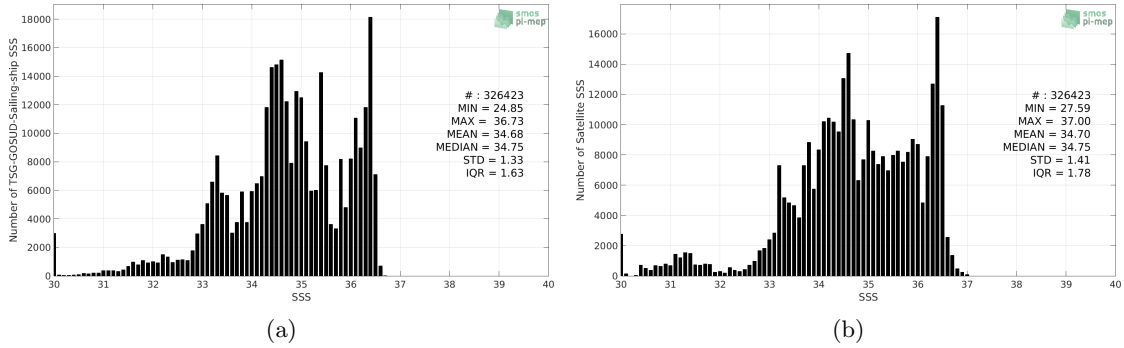
Figure 2: Histograms of SSS from TSG-GOSUD-Sailing-ship (a) and SMOS-L3-CATDS-CECOS-LOCEAN-V3-9DAYS-25KM (b) considering all match-up pairs per bins of 0.1 over the Pacific Ocean Pi-MEP region and for the full satellite product period.
