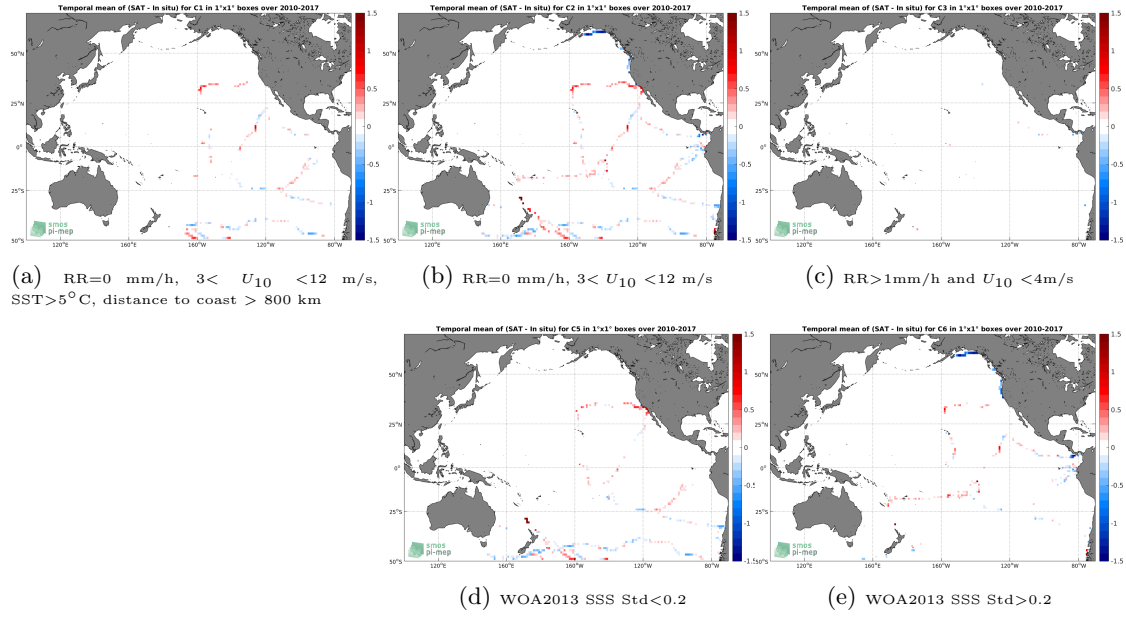
Figure 12: Temporal mean gridded over spatial boxes of size 1^\circ \times 1^\circ of \Delta SSS (SMOS-L3-CATDS-CECOS-LOCEAN-V3-9DAYS-25KM - TSG-GOSUD-Sailing-ship) for 5 different subdatasets corresponding to: RR=0 mm/h, 3 < U_{10} < 12 m/s, SST > 5^\circ C , distance to coast > 800 km (a), RR=0 mm/h, 3 < U_{10} < 12 m/s (b), RR > 1 mm/h and U_{10} < 4 m/s (c), WOA2013 SSS Std < 0.2 (d), WOA2013 SSS Std > 0.2 (e).
