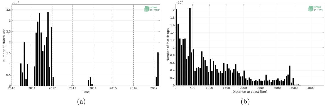
Figure 1: Number of match-ups between TSG-GOSUD-Sailing-ship and SMOS-L3-CATDS-CECOS-LOCEAN-V3-9DAYS-25KM SSS as a function of time (a) and as function of the distance to coast (b) over the Pacific Ocean Pi-MEP region and for the full satellite product period.
