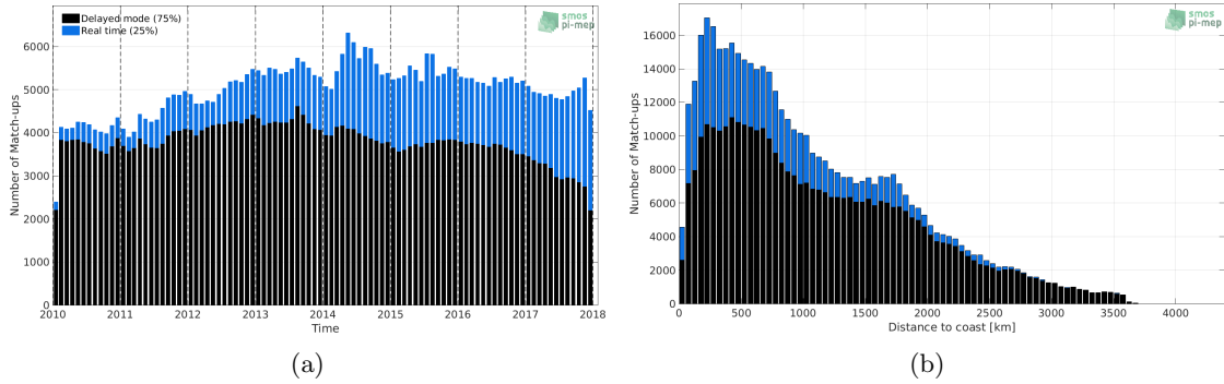
Figure 1: Number of match-ups between Argo and SMOS-L3-CATDS-CECOS-LOCEAN-V3-9DAYS-25KM SSS as a function of time (a) and as function of the distance to coast (b) over the Pacific Ocean Pi-MEP region and for the full satellite product period.
