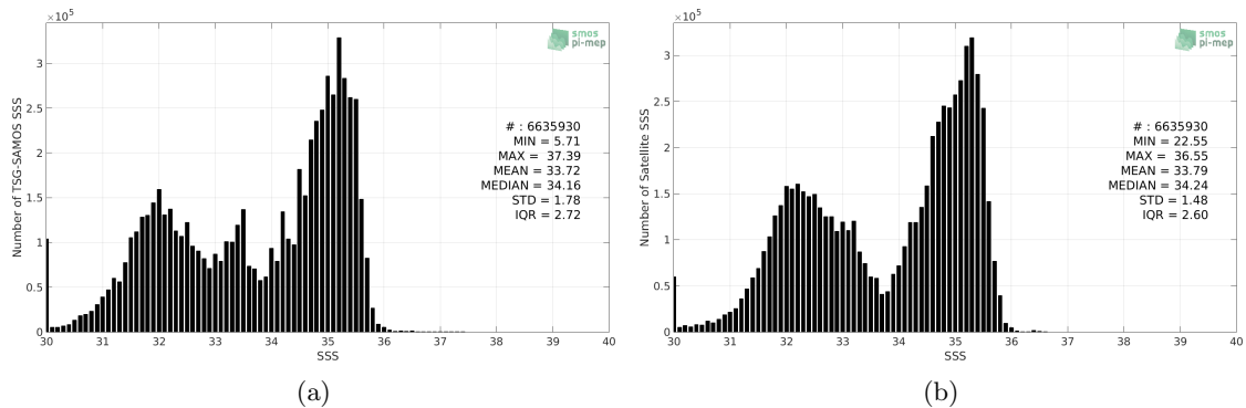
Figure 2: Histograms of SSS from TSG-SAMOS (a) and SMOS-L3-CATDS-CECOS-LOCEAN-V3-18DAYS-25KM (b) considering all match-up pairs per bins of 0.1 over the Pacific Ocean Pi-MEP region and for the full satellite product period.
