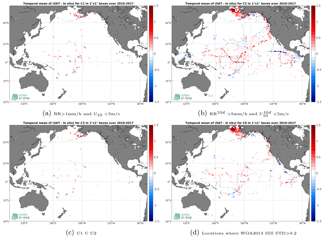
Figure 12: Temporal mean gridded over spatial boxes of size 1^\circ \times 1^\circ of \Delta SSS (SMOS-L3-CATDS-CECOS-LOCEAN-V3-18DAYS-25KM - TSG-SAMOS) for 4 different subdatasets corresponding to: RR > 1\text{mm/h} and U_{10} < 5\text{m/s} (a), RR^{10d} > 5\text{mm/h} and U_{10}^{10d} < 5\text{m/s} (b), C1 U C2 (c), Locations where WOA2013 SSS STD > 0.2 (d).
