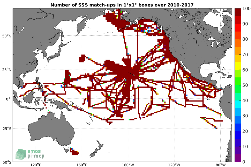
Figure 4: Number of SSS match-ups between TSG-SAMOS SSS and the SMOS-L3-CATDS-CECOS-LOCEAN-V3-18DAYS-25KM SSS product for the Pacific Ocean Pi-MEP region over 1^\circ \times 1^\circ boxes and for the full satellite product period.
