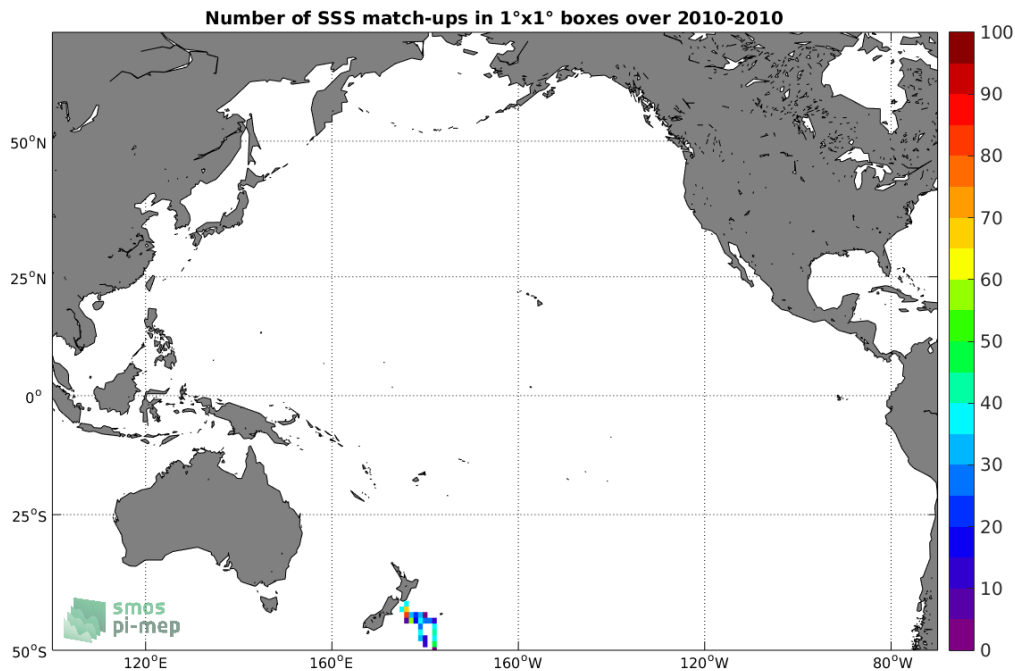
Figure 4: Number of SSS match-ups between TSG-POLARSTERN SSS and the SMOS-L3-CATDS-CECOS-LOCEAN-V3-18DAYS-25KM SSS product for the Pacific Ocean Pi-MEP region over 1°x1° boxes and for the full satellite product period.
