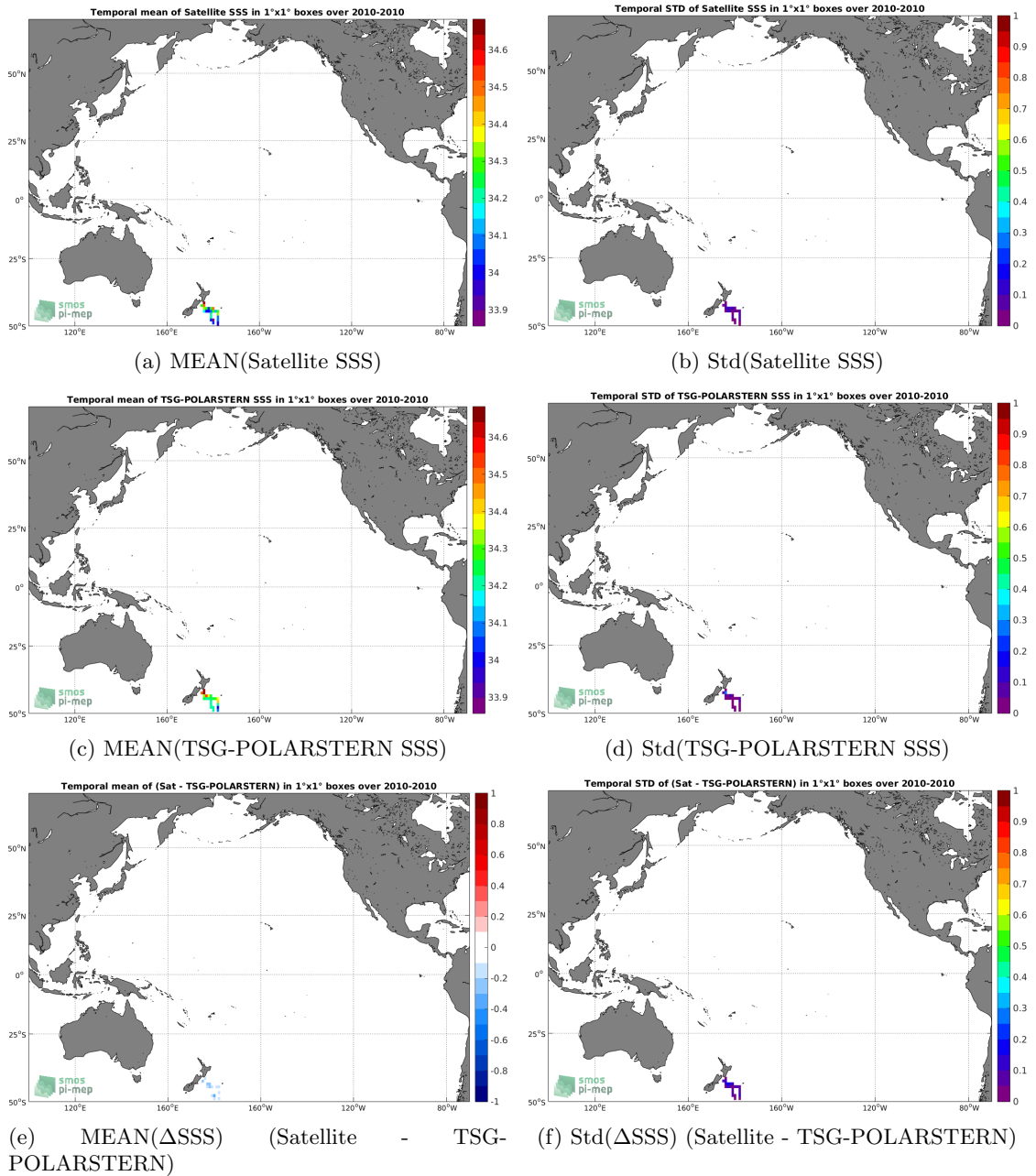
Figure 6: Temporal mean (left) and Std (right) of SSS from SMOS-L3-CATDS-CECOS-LOCEAN-V3-18DAYS-25KM (top), TSG-POLARSTERN (middle), and of \Delta SSS (Satellite - TSG-POLARSTERN). Only match-up pairs are used to generate these maps.
