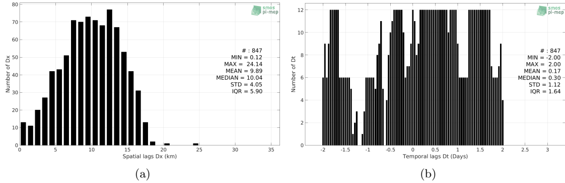
Figure 5: Histograms of the spatial (a) and temporal (b) lags between the time of the TSG-POLARSTERN measurements and the date of the corresponding SMOS-L3-CATDS-CECOS-LOCEAN-V3-18DAYS-25KM SSS product.
