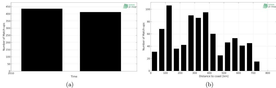
Figure 1: Number of match-ups between TSG-POLARSTERN and SMOS-L3-CATDS-CECOS-LOCEAN-V3-18DAYS-25KM SSS as a function of time (a) and as function of the distance to coast (b) over the Pacific Ocean Pi-MEP region and for the full satellite product period.
