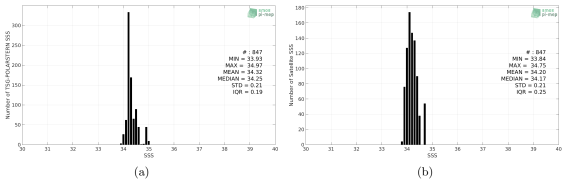
Figure 2: Histograms of SSS from TSG-POLARSTERN (a) and SMOS-L3-CATDS-CECOS-LOCEAN-V3-18DAYS-25KM (b) considering all match-up pairs per bins of 0.1 over the Pacific Ocean Pi-MEP region and for the full satellite product period.
