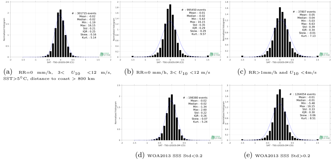
Figure 13: Normalized histogram of \Delta\text{SSS} (SMOS-L3-CATDS-CECOS-LOCEAN-V3-18DAYS-25KM - TSG-LEGOS-DM) for 5 different subdatasets corresponding to: RR=0 mm/h, 3 < U_{10} < 12 m/s, SST > 5^\circ\text{C} , distance to coast > 800 km (a), RR=0 mm/h, 3 < U_{10} < 12 m/s (b), RR > 1 mm/h and U_{10} < 4 m/s (c), WOA2013 SSS Std < 0.2 (d), WOA2013 SSS Std > 0.2 (e).
