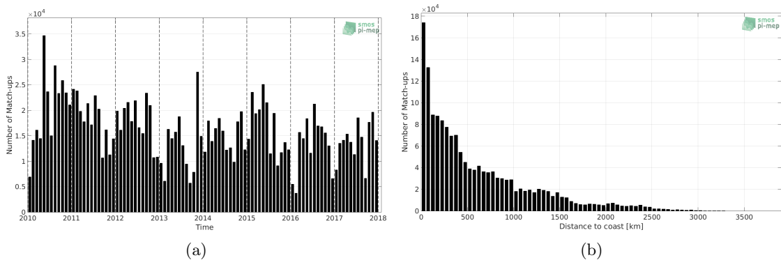
Figure 1: Number of match-ups between TSG-LEGOS-DM and SMOS-L3-CATDS-CECOS-LOCEAN-V3-18DAYS-25KM SSS as a function of time (a) and as function of the distance to coast (b) over the Pacific Ocean Pi-MEP region and for the full satellite product period.
