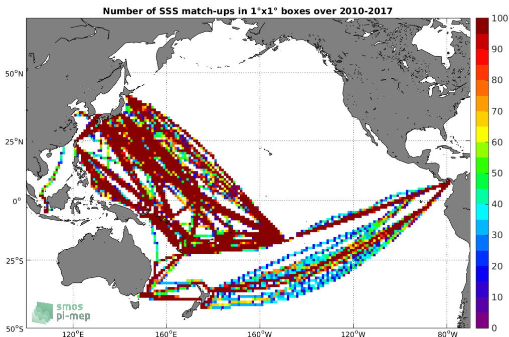
Figure 4: Number of SSS match-ups between TSG-LEGOS-DM SSS and the SMOS-L3-CATDS-CECOS-LOCEAN-V3-18DAYS-25KM SSS product for the Pacific Ocean Pi-MEP region over 1^\circ \times 1^\circ boxes and for the full satellite product period.
