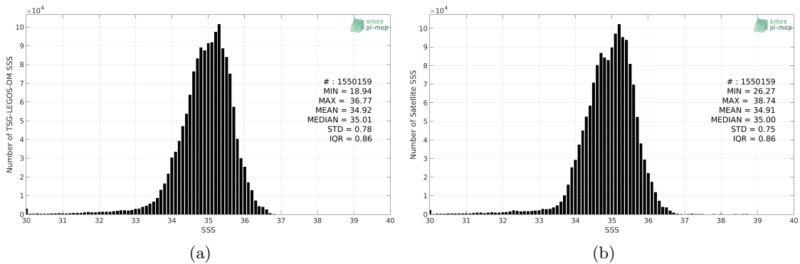
Figure 2: Histograms of SSS from TSG-LEGOS-DM (a) and SMOS-L3-CATDS-CECOS-LOCEAN-V3-18DAYS-25KM (b) considering all match-up pairs per bins of 0.1 over the Pacific Ocean Pi-MEP region and for the full satellite product period.
