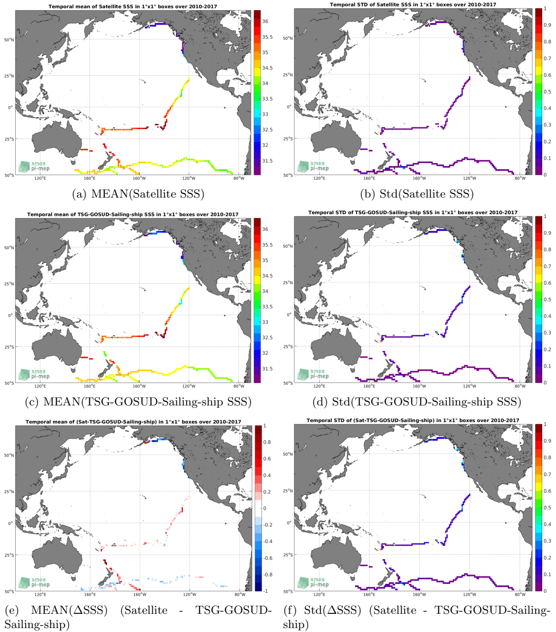
Figure 6: Temporal mean (left) and Std (right) of SSS from SMOS-L3-CATDS-CECOS-LOCEAN-V3-18DAYS-25KM (top), TSG-GOSUD-Sailing-ship (middle), and of \Delta SSS (Satellite - TSG-GOSUD-Sailing-ship). Only match-up pairs are used to generate these maps.
