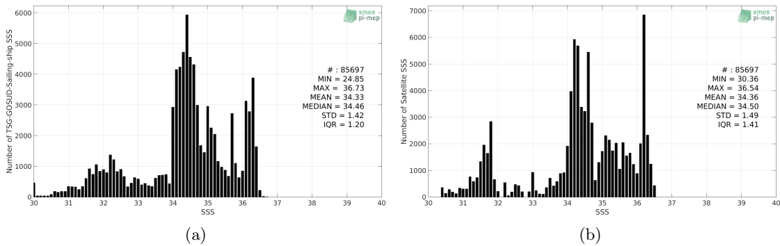
Figure 2: Histograms of SSS from TSG-GOSUD-Sailing-ship (a) and SMOS-L3-CATDS-CECOS-LOCEAN-V3-18DAYS-25KM (b) considering all match-up pairs per bins of 0.1 over the Pacific Ocean Pi-MEP region and for the full satellite product period.
