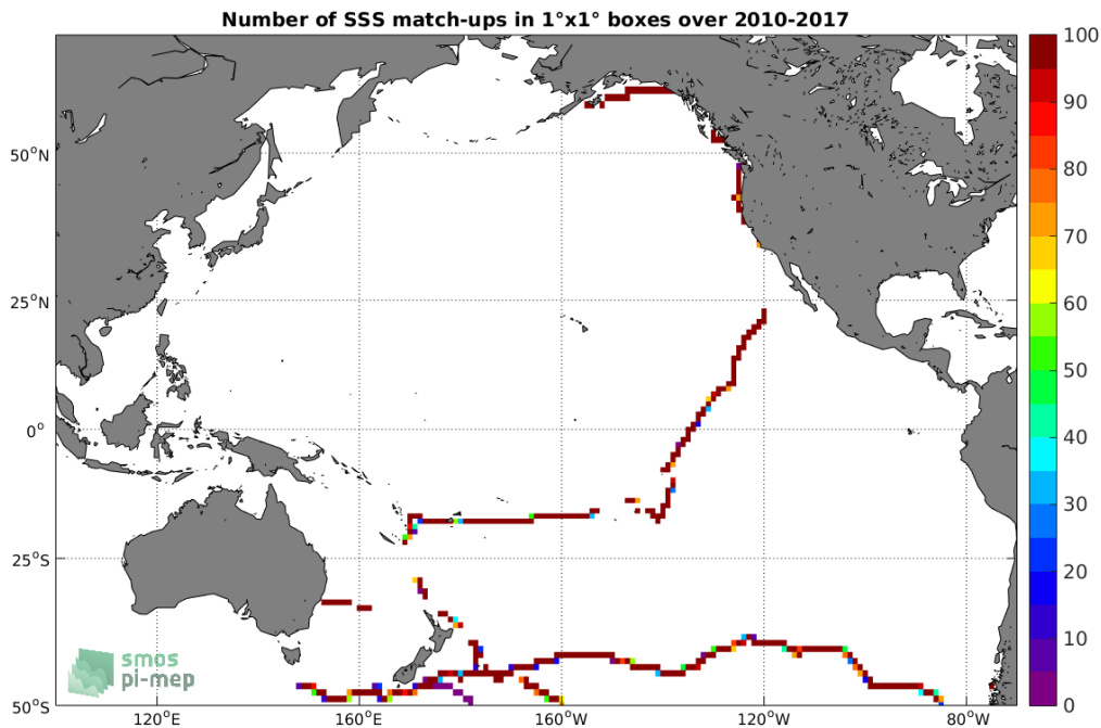
Figure 4: Number of SSS match-ups between TSG-GOSUD-Sailing-ship SSS and the SMOS-L3-CATDS-CECOS-LOCEAN-V3-18DAYS-25KM SSS product for the Pacific Ocean Pi-MEP region over 1^\circ \times 1^\circ boxes and for the full satellite product period.
