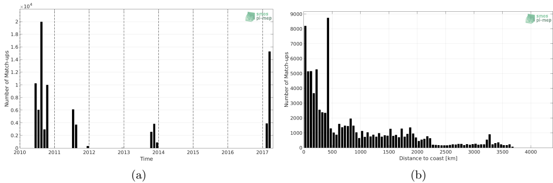
Figure 1: Number of match-ups between TSG-GOSUD-Sailing-ship and SMOS-L3-CATDS-CECOS-LOCEAN-V3-18DAYS-25KM SSS as a function of time (a) and as function of the distance to coast (b) over the Pacific Ocean Pi-MEP region and for the full satellite product period.
