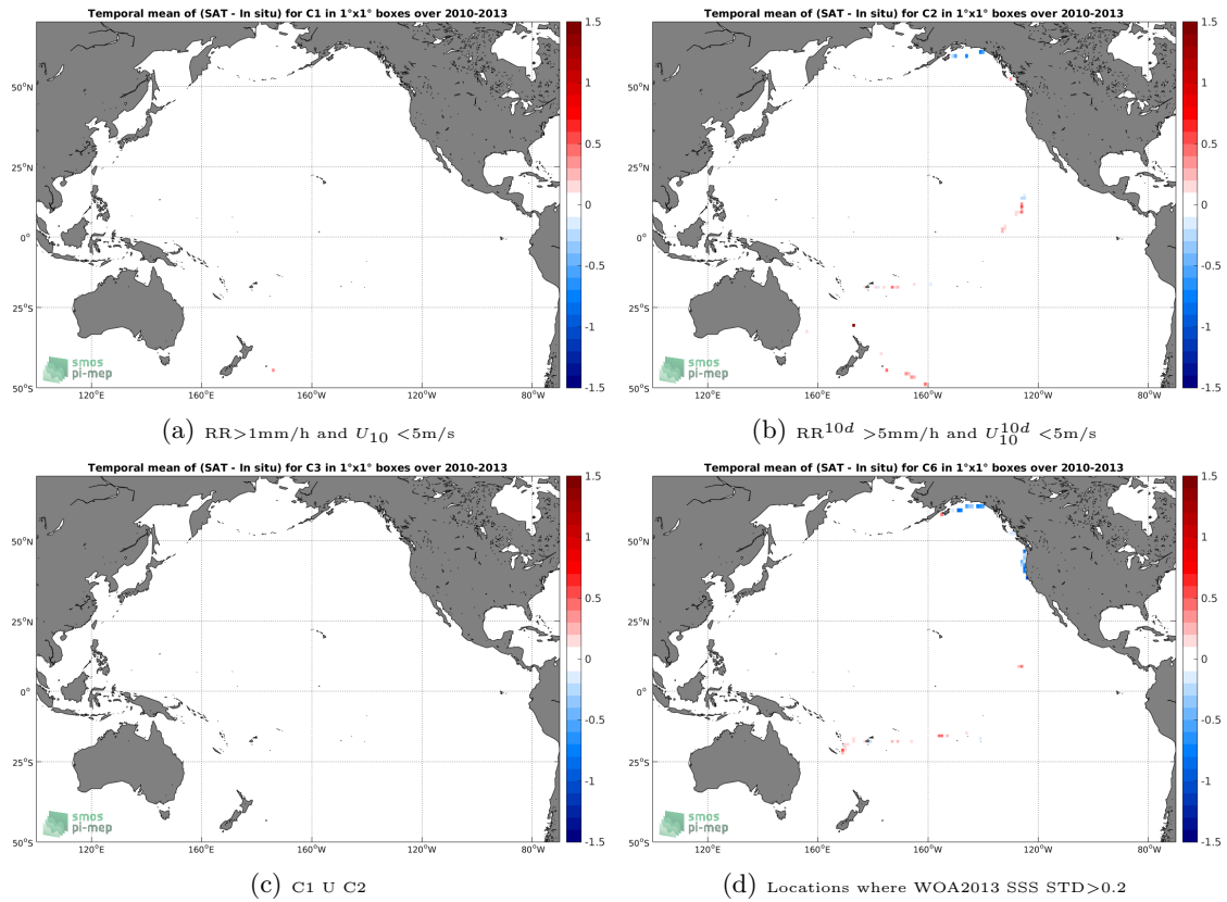
Figure 12: Temporal mean gridded over spatial boxes of size 1^\circ \times 1^\circ of \Delta SSS (SMOS-L3-CATDS-CECOS-LOCEAN-V3-18DAYS-25KM - TSG-GOSUD-Sailing-ship) for 4 different subdatasets corresponding to: RR > 1\text{mm/h} and U_{10} < 5\text{m/s} (a), RR^{10d} > 5\text{mm/h} and U_{10}^{10d} < 5\text{m/s} (b), C1 U C2 (c), Locations where WOA2013 SSS STD > 0.2 (d).
