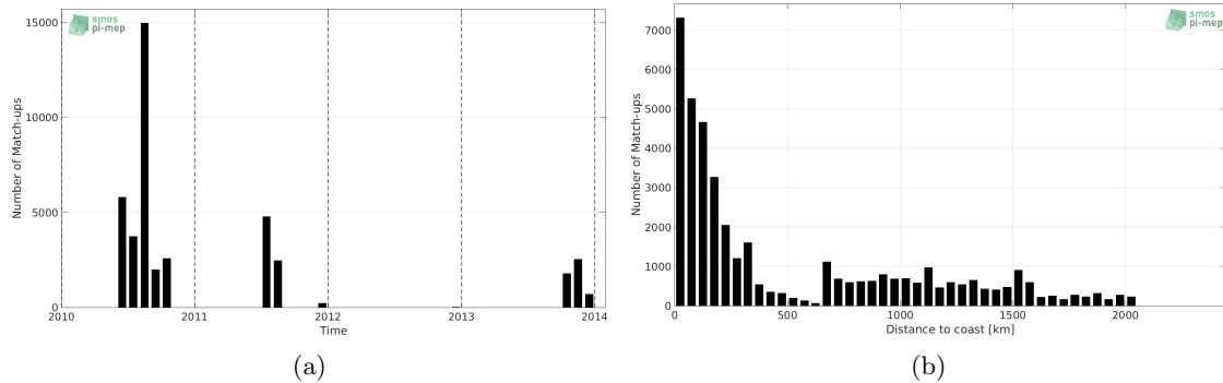
Figure 1: Number of match-ups between TSG-GOSUD-Sailing-ship and SMOS-L3-CATDS-CECOS-LOCEAN-V3-18DAYS-25KM SSS as a function of time (a) and as function of the distance to coast (b) over the Pacific Ocean Pi-MEP region and for the full satellite product period.
