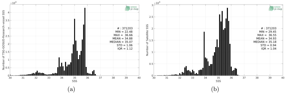
Figure 2: Histograms of SSS from TSG-GOSUD-Research-vessel (a) and SMOS-L3-CATDS-CECOS-LOCEAN-V3-18DAYS-25KM (b) considering all match-up pairs per bins of 0.1 over the Pacific Ocean Pi-MEP region and for the full satellite product period.
