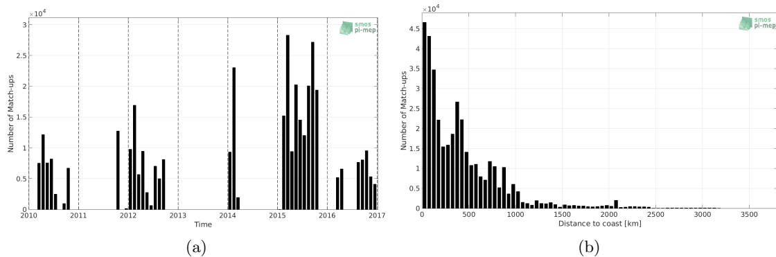
Figure 1: Number of match-ups between TSG-GOSUD-Research-vessel and SMOS-L3-CATDS-CECOS-LOCEAN-V3-18DAYS-25KM SSS as a function of time (a) and as function of the distance to coast (b) over the Pacific Ocean Pi-MEP region and for the full satellite product period.
