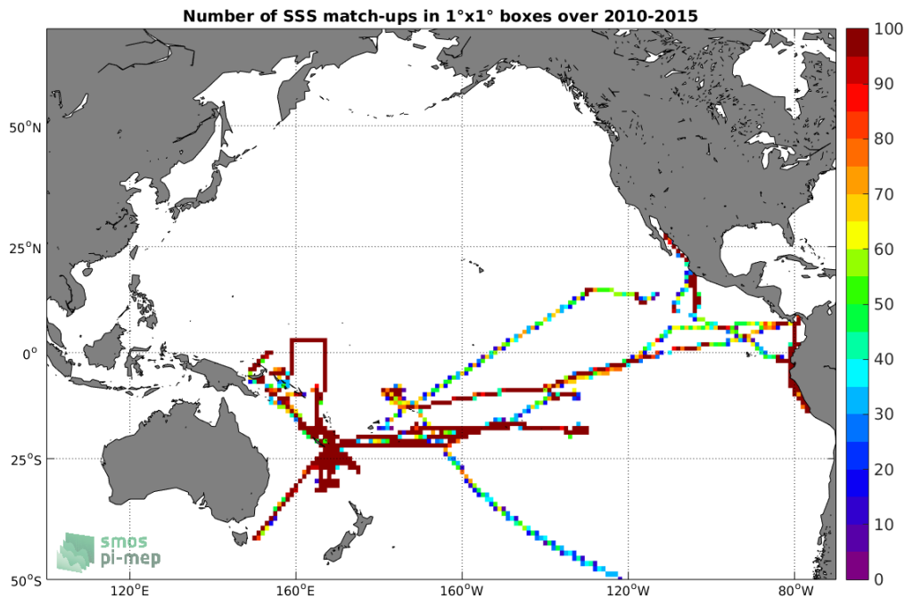
Figure 4: Number of SSS match-ups between TSG-GOSUD-Research-vessel SSS and the SMOS-L3-CATDS-CECOS-LOCEAN-V3-18DAYS-25KM SSS product for the Pacific Ocean Pi-MEP region over 1^\circ \times 1^\circ boxes and for the full satellite product period.
