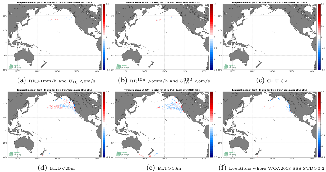
Figure 12: Temporal mean gridded over spatial boxes of size 1^\circ \times 1^\circ of \Delta\text{SSS} (SMOS-L3-CATDS-CECOS-LOCEAN-V3-18DAYS-25KM - Sea mammals) for 6 different subdatasets corresponding to: \text{RR} > 1\text{mm/h} and U_{10} < 5\text{m/s} (a), \text{RR}^{10d} > 5\text{mm/h} and U_{10}^{10d} < 5\text{m/s} (b), C1 U C2 (c), \text{MLD} < 20\text{m} (d), \text{BLT} > 10\text{m} (e), Locations where WOA2013 SSS STD > 0.2 (f).
