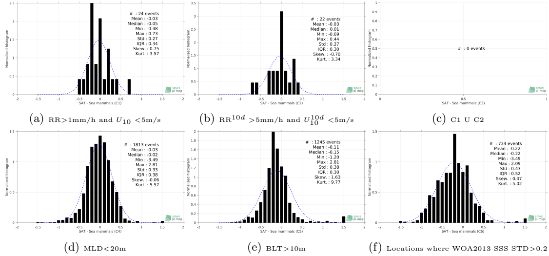
Figure 13: Normalized histogram of \Delta SSS (SMOS-L3-CATDS-CECOS-LOCEAN-V3-18DAYS-25KM - Sea mammals) for 6 different subdatasets corresponding to: RR > 1mm/h and U_{10} < 5m/s (a), RR^{10d} > 5mm/h and U_{10}^{10d} < 5m/s (b), C1 U C2 (c), MLD < 20m (d), BLT > 10m (e), Locations where WOA2013 SSS STD > 0.2 (f).
