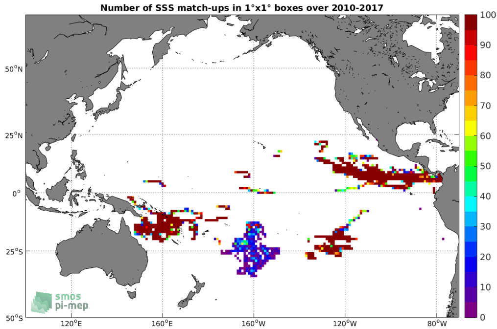
Figure 3: Number of SSS match-ups between Surface drifters SSS and the SMOS-L3-CATDS-CECOS-LOCEAN-V3-18DAYS-25KM SSS product for the Pacific Ocean Pi-MEP region over 1°x1° boxes and for the full satellite product period.
