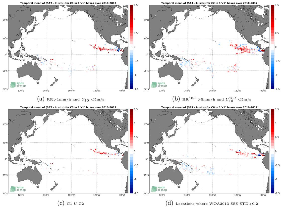
Figure 11: Temporal mean gridded over spatial boxes of size 1^\circ \times 1^\circ of \Delta SSS (SMOS-L3-CATDS-CECOS-LOCEAN-V3-18DAYS-25KM - Surface drifters) for 4 different subdatasets corresponding to: RR > 1\text{mm/h} and U_{10} < 5\text{m/s} (a), RR^{10d} > 5\text{mm/h} and U_{10}^{10d} < 5\text{m/s} (b), C1 U C2 (c), Locations where WOA2013 SSS STD > 0.2 (d).
