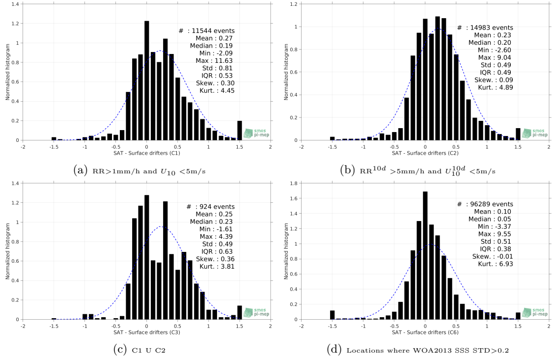
Figure 12: Normalized histogram of \Delta SSS (SMOS-L3-CATDS-CECOS-LOCEAN-V3-18DAYS-25KM - Surface drifters) for 6 different subdatasets corresponding to: RR > 1mm/h and U_{10} < 5 m/s (a), RR^{10d} > 5 mm/h and U_{10}^{10d} < 5 m/s (b), C1 U C2 (c), Locations where WOA2013 SSS STD > 0.2 (d).
