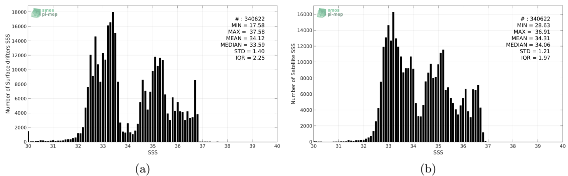
Figure 2: Histograms of SSS from Surface drifters (a) and SMOS-L3-CATDS-CECOS-LOCEAN-V3-18DAYS-25KM (b) considering all match-up pairs per bins of 0.1 over the Pacific Ocean Pi-MEP region and for the full satellite product period.
