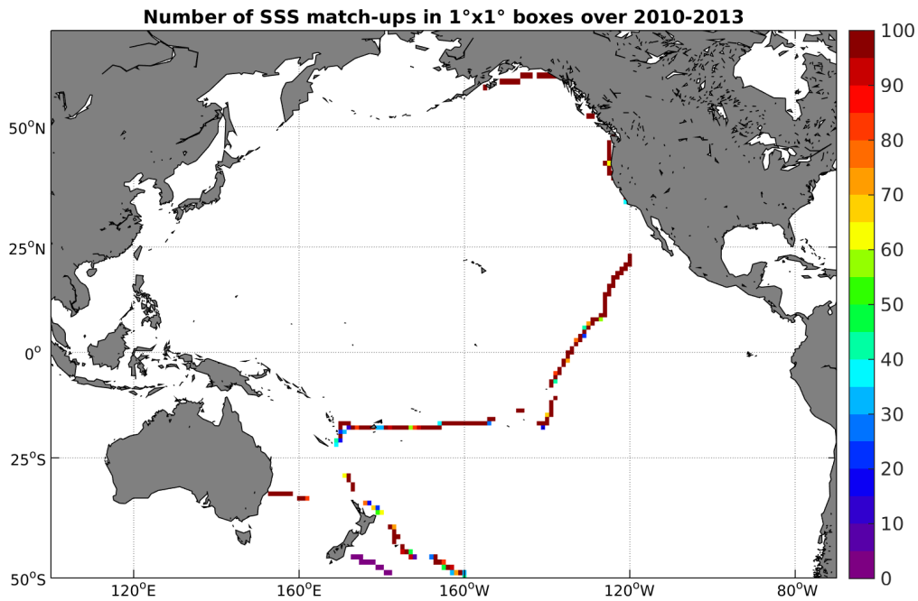
Figure 4: Number of SSS match-ups between TSG-GOSUD-Sailing-ship SSS and the SMOS-L3-CATDS-CECOS-LOCEAN-V2-9DAYS-25KM SSS product for the Pacific Ocean Pi-MEP region over 1^\circ \times 1^\circ boxes and for the full satellite product period.
