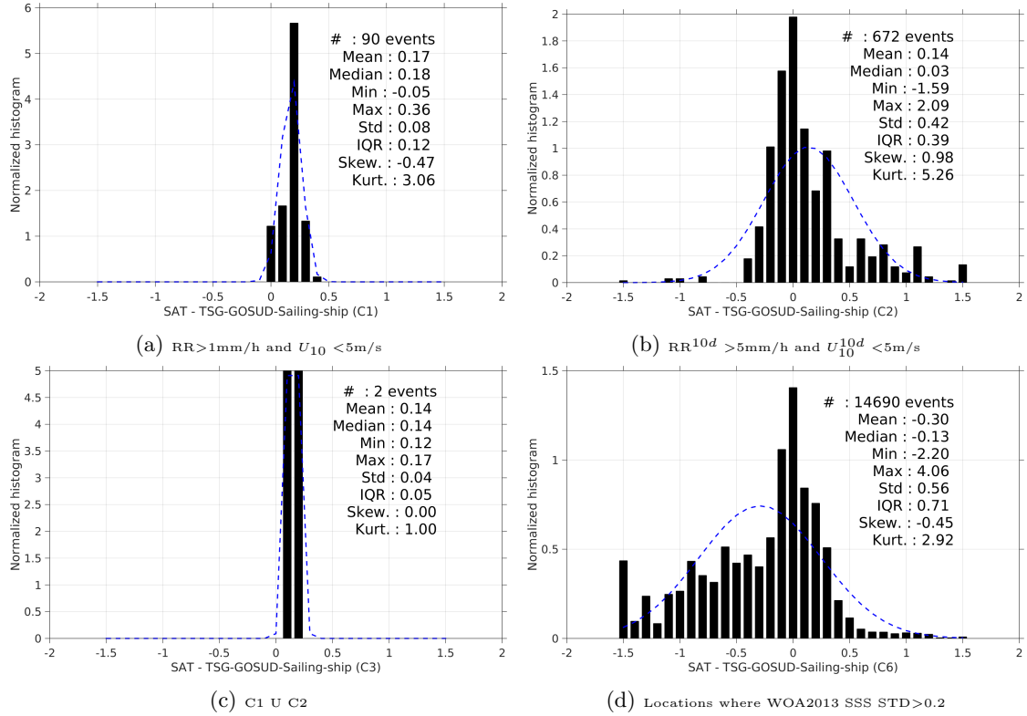
Figure 13: Normalized histogram of \Delta\text{SSS} (SMOS-L3-CATDS-CECOS-LOCEAN-V2-9DAYS-25KM - TSG-GOSUD-Sailing-ship) for 6 different subdatasets corresponding to: RR > 1mm/h and U_{10} < 5\text{m/s} (a), RR^{10d} > 5\text{mm/h} and U_{10}^{10d} < 5\text{m/s} (b), C1 U C2 (c), Locations where WOA2013 SSS STD > 0.2 (d).
