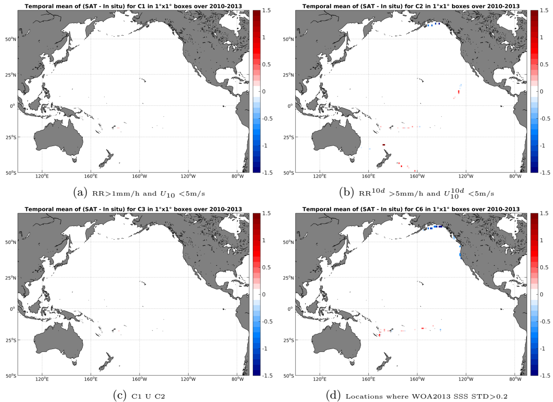
Figure 12: Temporal mean gridded over spatial boxes of size 1°x1° of \Delta SSS (SMOS-L3-CATDS-CECOS-LOCEAN-V2-9DAYS-25KM - TSG-GOSUD-Sailing-ship) for 4 different subdatasets corresponding to:RR>1mm/h and U_{10} < 5\text{m/s} (a), RR^{10d} > 5\text{mm/h} and U_{10}^{10d} < 5\text{m/s} (b), C1 U C2 (c),Locations where WOA2013 SSS STD>0.2 (d).
