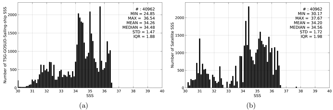
Figure 2: Histograms of SSS from TSG-GOSUD-Sailing-ship (a) and SMOS-L3-CATDS-CECOS-LOCEAN-V2-9DAYS-25KM (b) considering all match-up pairs per bins of 0.1 over the Pacific Ocean Pi-MEP region and for the full satellite product period.
