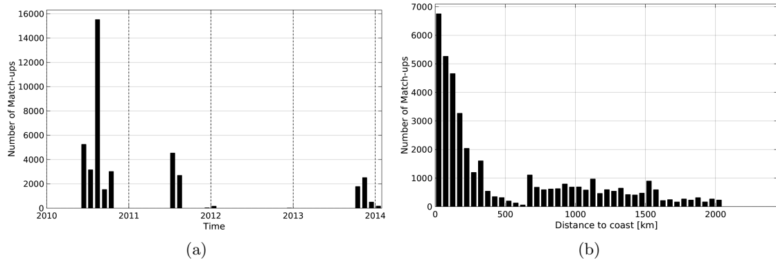
Figure 1: Number of match-ups between TSG-GOSUD-Sailing-ship and SMOS-L3-CATDS-CECOS-LOCEAN-V2-9DAYS-25KM SSS as a function of time (a) and as function of the distance to coast (b) over the Pacific Ocean Pi-MEP region and for the full satellite product period.
