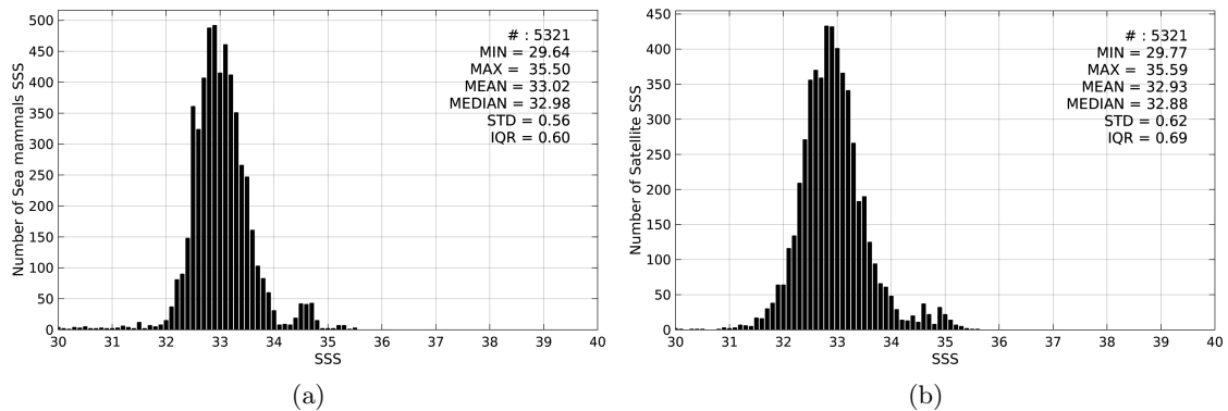
Figure 2: Histograms of SSS from Sea mammals (a) and SMOS-L3-CATDS-CECOS-LOCEAN-V2-9DAYS-25KM (b) considering all match-up pairs per bins of 0.1 over the Pacific Ocean Pi-MEP region and for the full satellite product period.
