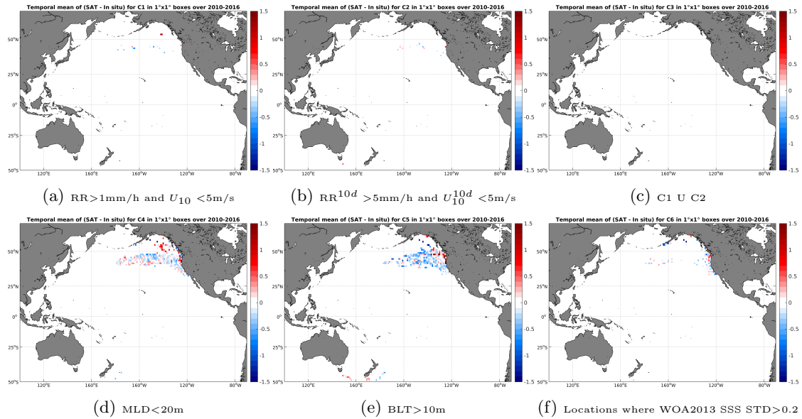
Figure 12: Temporal mean gridded over spatial boxes of size 1^\circ \times 1^\circ of \Delta SSS (SMOS-L3-CATDS-CECOS-LOCEAN-V2-9DAYS-25KM - Sea mammals) for 6 different subdatasets corresponding to: RR > 1\text{mm/h} and U_{10} < 5\text{m/s} (a), RR^{10d} > 5\text{mm/h} and U_{10}^{10d} < 5\text{m/s} (b), C1 U C2 (c), MLD < 20\text{m} (d), BLT > 10\text{m} (e), Locations where WOA2013 SSS STD > 0.2 (f).
