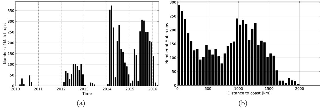
Figure 1: Number of match-ups between Sea mammals and SMOS-L3-CATDS-CECOS-LOCEAN-V2-9DAYS-25KM SSS as a function of time (a) and as function of the distance to coast (b) over the Pacific Ocean Pi-MEP region and for the full satellite product period.
