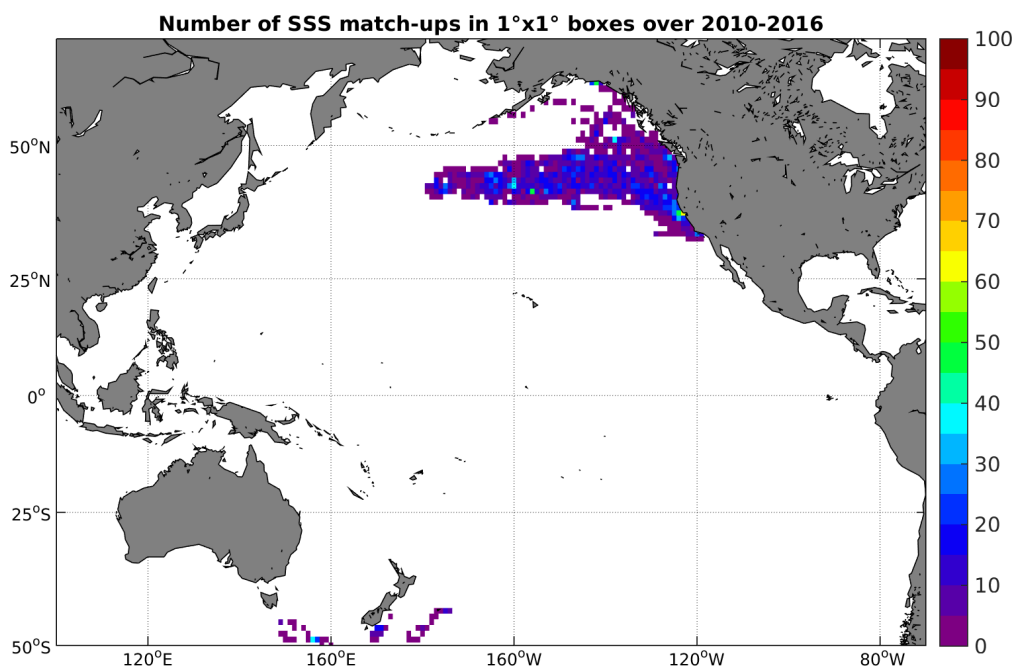
Figure 4: Number of SSS match-ups between Sea mammals SSS and the SMOS-L3-CATDS-CECOS-LOCEAN-V2-9DAYS-25KM SSS product for the Pacific Ocean Pi-MEP region over 1°x1° boxes and for the full satellite product period.
