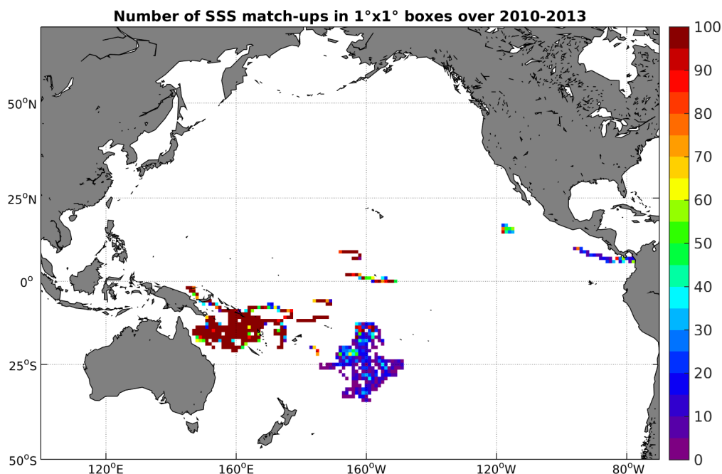
Figure 3: Number of SSS match-ups between Surface drifters SSS and the SMOS-L3-CATDS-CECOS-LOCEAN-V2-9DAYS-25KM SSS product for the Pacific Ocean Pi-MEP region over 1°x1° boxes and for the full satellite product period.
