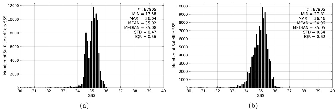
Figure 2: Histograms of SSS from Surface drifters (a) and SMOS-L3-CATDS-CECOS-LOCEAN-V2-9DAYS-25KM (b) considering all match-up pairs per bins of 0.1 over the Pacific Ocean Pi-MEP region and for the full satellite product period.
