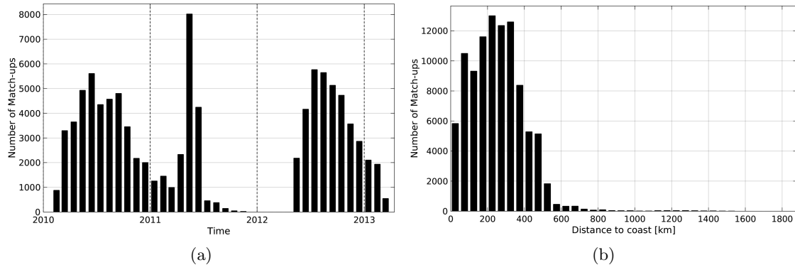
Figure 1: Number of match-ups between Surface drifters and SMOS-L3-CATDS-CECOS-LOCEAN-V2-9DAYS-25KM SSS as a function of time (a) and as function of the distance to coast (b) over the Pacific Ocean Pi-MEP region and for the full satellite product period.
