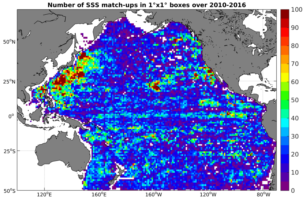
Figure 4: Number of SSS match-ups between Argo SSS and the SMOS-L3-CATDS-CECOS-LOCEAN-V2-9DAYS-25KM SSS product for the Pacific Ocean Pi-MEP region over 1^\circ \times 1^\circ boxes and for the full satellite product period.
