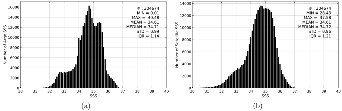
Figure 2: Histograms of SSS from Argo (a) and SMOS-L3-CATDS-CECOS-LOCEAN-V2-9DAYS-25KM (b) considering all match-up pairs per bins of 0.1 over the Pacific Ocean Pi-MEP region and for the full satellite product period.
