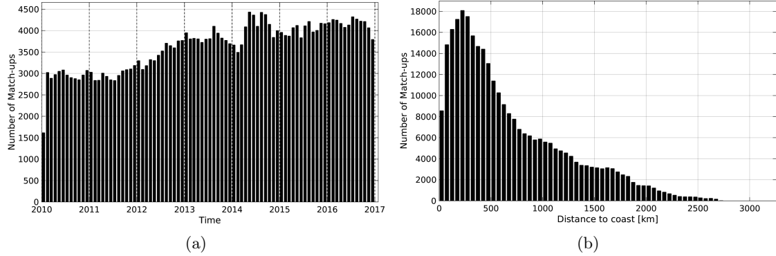
Figure 1: Number of match-ups between Argo and SMOS-L3-CATDS-CECOS-LOCEAN-V2-9DAYS-25KM SSS as a function of time (a) and as function of the distance to coast (b) over the Pacific Ocean Pi-MEP region and for the full satellite product period.
