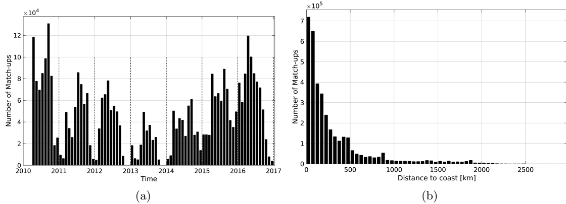
Figure 1: Number of match-ups between TSG-SAMOS and SMOS-L3-CATDS-CECOS-LOCEAN-V2-18DAYS-25KM SSS as a function of time (a) and as function of the distance to coast (b) over the Pacific Ocean Pi-MEP region and for the full satellite product period.
