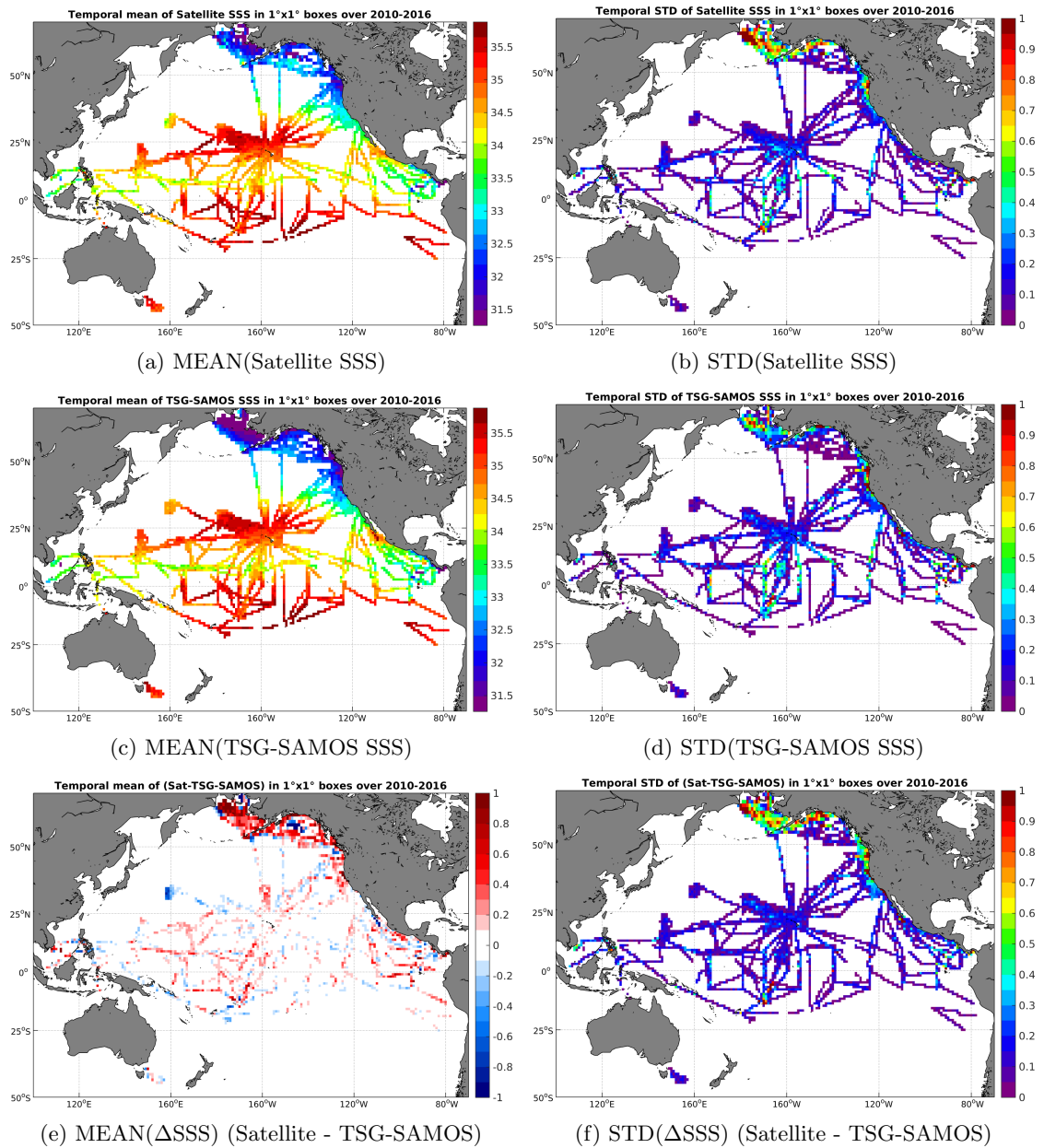
Figure 6: Temporal mean (left) and STD (right) of SSS from SMOS-L3-CATDS-CECOS-LOCEAN-V2-18DAYS-25KM (top), TSG-SAMOS (middle), and of \Delta SSS (Satellite - TSG-SAMOS). Only match-up pairs are used to generate these maps.
