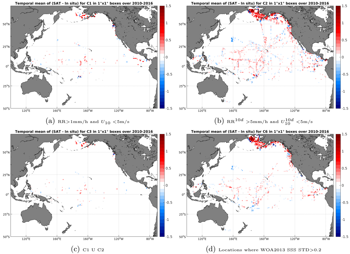
Figure 12: Temporal mean gridded over spatial boxes of size 1^\circ \times 1^\circ of \Delta SSS (SMOS-L3-CATDS-CECOS-LOCEAN-V2-18DAYS-25KM - TSG-SAMOS) for 4 different subdatasets corresponding to: RR > 1\text{mm/h} and U_{10} < 5\text{m/s} (a), RR^{10d} > 5\text{mm/h} and U_{10}^{10d} < 5\text{m/s} (b), C1 U C2 (c), Locations where WOA2013 SSS STD > 0.2 (d).
