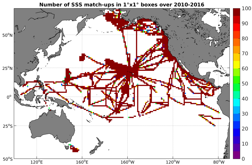
Figure 4: Number of SSS match-ups between TSG-SAMOS SSS and the SMOS-L3-CATDS-CECOS-LOCEAN-V2-18DAYS-25KM SSS product for the Pacific Ocean Pi-MEP region over 1^\circ \times 1^\circ boxes and for the full satellite product period.
