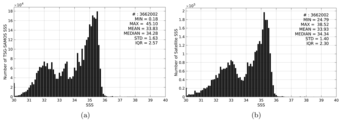
Figure 2: Histograms of SSS from TSG-SAMOS (a) and SMOS-L3-CATDS-CECOS-LOCEAN-V2-18DAYS-25KM (b) considering all match-up pairs per bins of 0.1 over the Pacific Ocean Pi-MEP region and for the full satellite product period.
