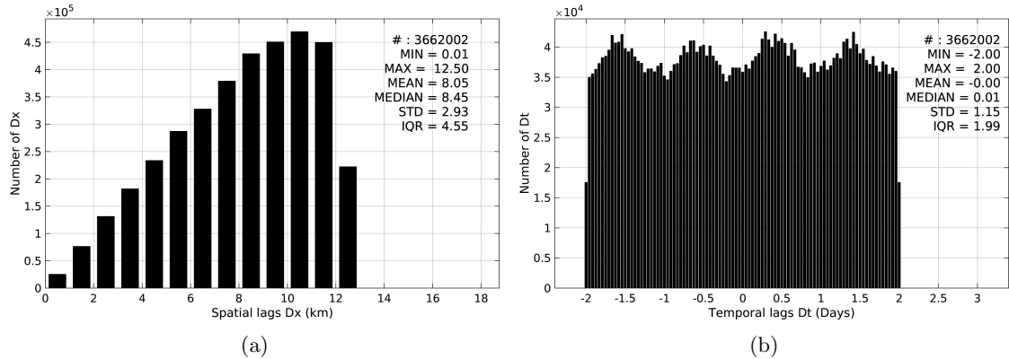
Figure 5: Histograms of the spatial (a) and temporal (b) lags between the time of the TSG-SAMOS measurements and the date of the corresponding SMOS-L3-CATDS-CECOS-LOCEAN-V2-18DAYS-25KM SSS product.
