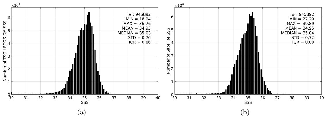
Figure 2: Histograms of SSS from TSG-LEGOS-DM (a) and SMOS-L3-CATDS-CECOS-LOCEAN-V2-18DAYS-25KM (b) considering all match-up pairs per bins of 0.1 over the Pacific Ocean Pi-MEP region and for the full satellite product period.
