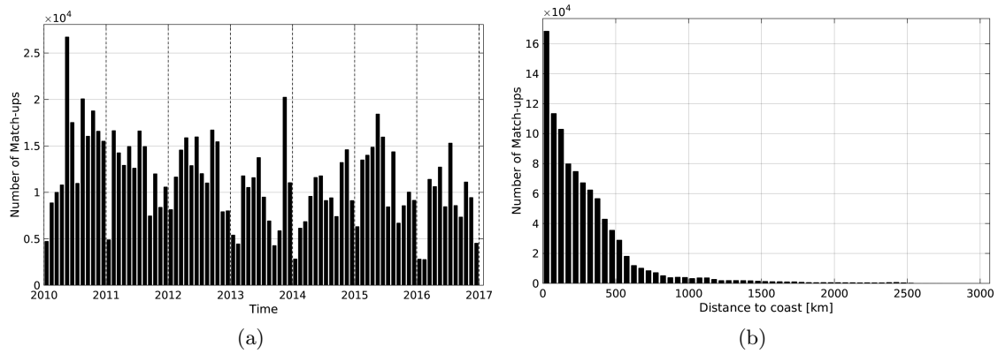
Figure 1: Number of match-ups between TSG-LEGOS-DM and SMOS-L3-CATDS-CECOS-LOCEAN-V2-18DAYS-25KM SSS as a function of time (a) and as function of the distance to coast (b) over the Pacific Ocean Pi-MEP region and for the full satellite product period.
