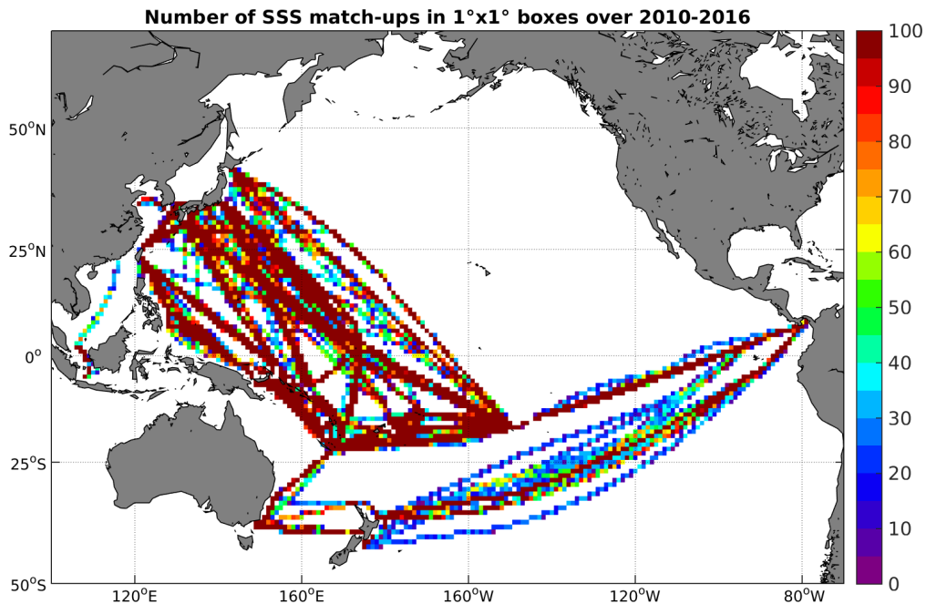
Figure 4: Number of SSS match-ups between TSG-LEGOS-DM SSS and the SMOS-L3-CATDS-CECOS-LOCEAN-V2-18DAYS-25KM SSS product for the Pacific Ocean Pi-MEP region over 1^\circ \times 1^\circ boxes and for the full satellite product period.
