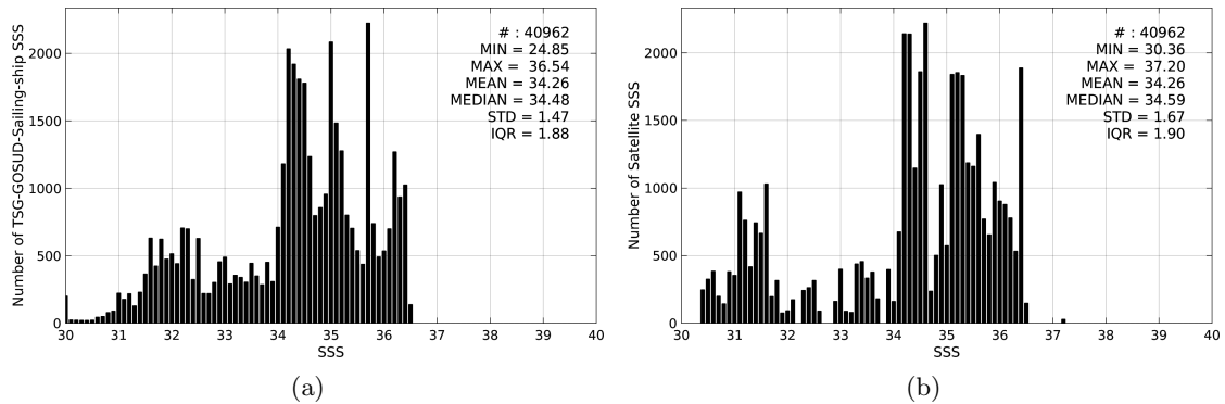
Figure 2: Histograms of SSS from TSG-GOSUD-Sailing-ship (a) and SMOS-L3-CATDS-CECOS-LOCEAN-V2-18DAYS-25KM (b) considering all match-up pairs per bins of 0.1 over the Pacific Ocean Pi-MEP region and for the full satellite product period.
