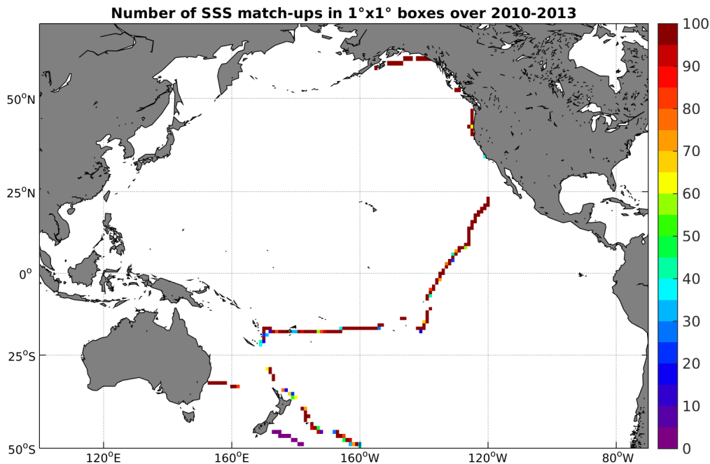
Figure 4: Number of SSS match-ups between TSG-GOSUD-Sailing-ship SSS and the SMOS-L3-CATDS-CECOS-LOCEAN-V2-18DAYS-25KM SSS product for the Pacific Ocean Pi-MEP region over 1^\circ \times 1^\circ boxes and for the full satellite product period.
