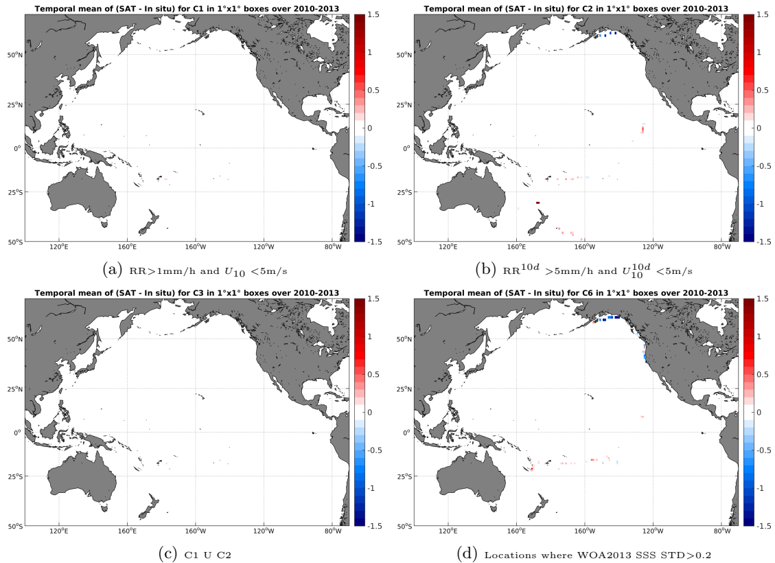
Figure 12: Temporal mean gridded over spatial boxes of size 1^\circ \times 1^\circ of \Delta SSS (SMOS-L3-CATDS-CECOS-LOCEAN-V2-18DAYS-25KM - TSG-GOSUD-Sailing-ship) for 4 different subdatasets corresponding to: RR > 1mm/h and U_{10} < 5 m/s (a), RR 10d > 5mm/h and U_{10}^{10d} < 5 m/s (b), C1 U C2 (c), Locations where WOA2013 SSS STD > 0.2 (d).
