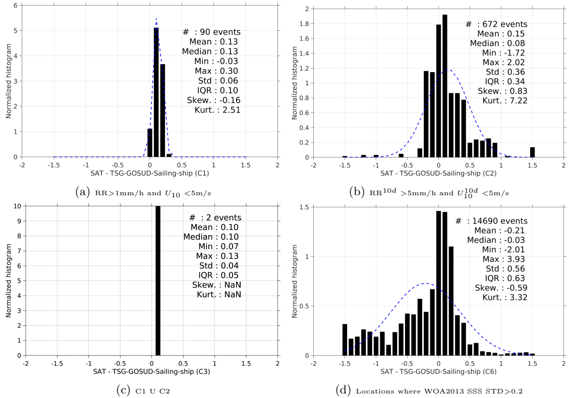
Figure 13: Normalized histogram of \Delta\text{SSS} (SMOS-L3-CATDS-CECOS-LOCEAN-V2-18DAYS-25KM - TSG-GOSUD-Sailing-ship) for 6 different subdatasets corresponding to: RR > 1mm/h and U_{10} < 5\text{m/s} (a), RR^{10d} > 5\text{mm/h} and U_{10}^{10d} < 5\text{m/s} (b), C1 U C2 (c), Locations where WOA2013 SSS STD > 0.2 (d).
