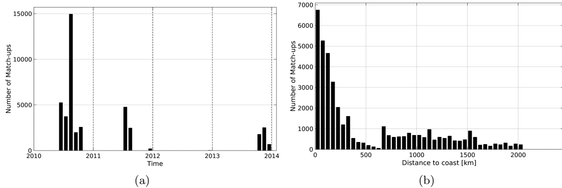
Figure 1: Number of match-ups between TSG-GOSUD-Sailing-ship and SMOS-L3-CATDS-CECOS-LOCEAN-V2-18DAYS-25KM SSS as a function of time (a) and as function of the distance to coast (b) over the Pacific Ocean Pi-MEP region and for the full satellite product period.
