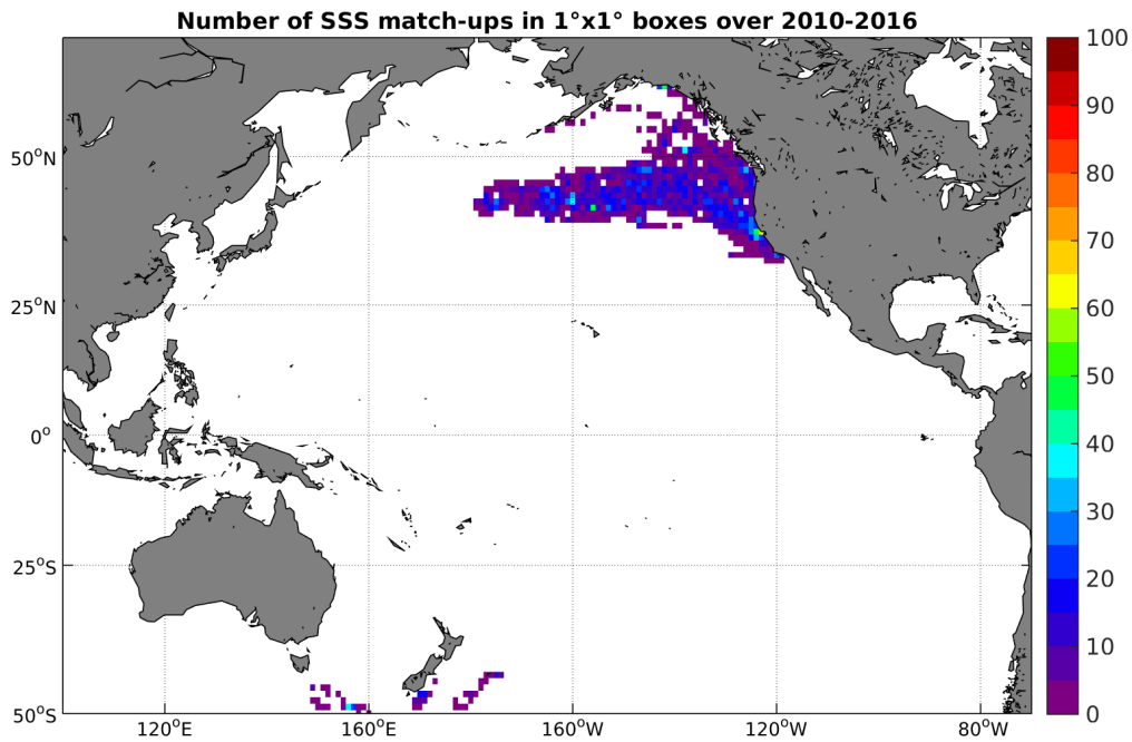
Figure 4: Number of SSS match-ups between Sea mammals SSS and the SMOS-L3-CATDS-CECOS-LOCEAN-V2-18DAYS-25KM SSS product for the Pacific Ocean Pi-MEP region over 1°x1° boxes and for the full satellite product period.
