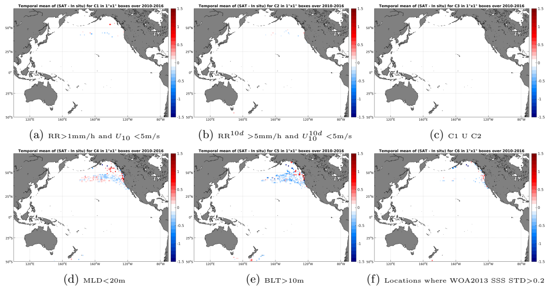
Figure 12: Temporal mean gridded over spatial boxes of size 1^\circ \times 1^\circ of \Delta SSS (SMOS-L3-CATDS-CECOS-LOCEAN-V2-18DAYS-25KM - Sea mammals) for 6 different subdatasets corresponding to: RR > 1\text{mm/h} and U_{10} < 5\text{m/s} (a), RR^{10d} > 5\text{mm/h} and U_{10}^{10d} < 5\text{m/s} (b), C1 U C2 (c), MLD < 20\text{m} (d), BLT > 10\text{m} (e), Locations where WOA2013 SSS STD > 0.2 (f).
