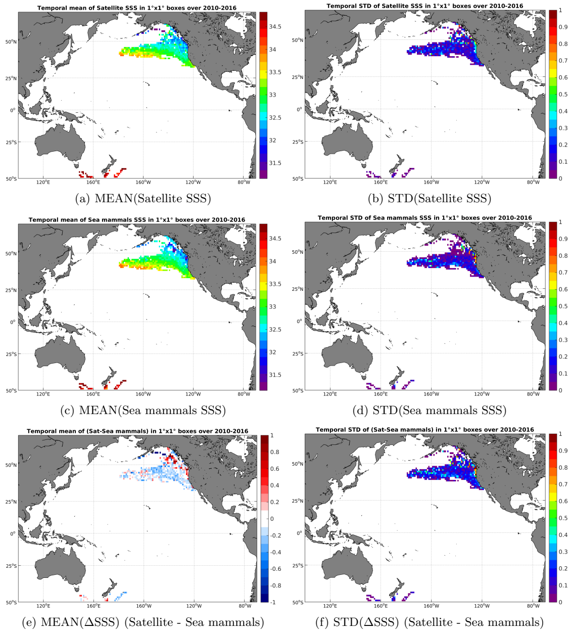
Figure 6: Temporal mean (left) and STD (right) of SSS from SMOS-L3-CATDS-CECOS-LOCEAN-V2-18DAYS-25KM (top), Sea mammals (middle), and of \Delta SSS (Satellite - Sea mammals). Only match-up pairs are used to generate these maps.
