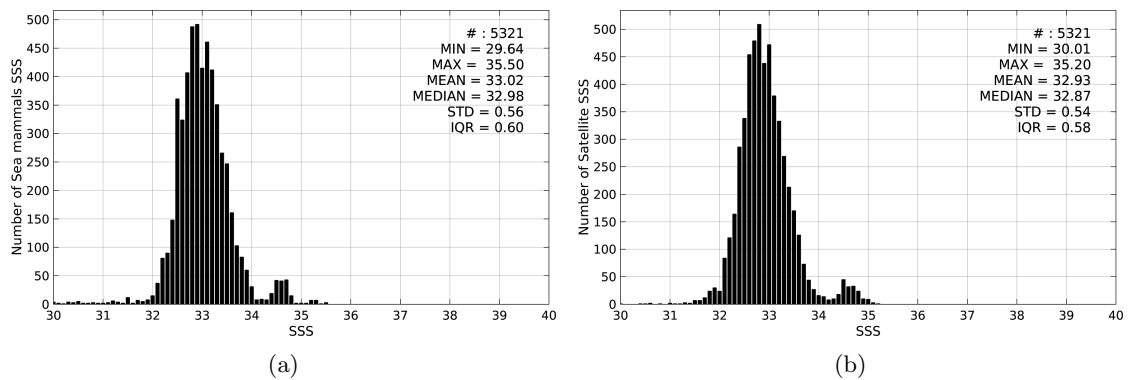
Figure 2: Histograms of SSS from Sea mammals (a) and SMOS-L3-CATDS-CECOS-LOCEAN-V2-18DAYS-25KM (b) considering all match-up pairs per bins of 0.1 over the Pacific Ocean Pi-MEP region and for the full satellite product period.
