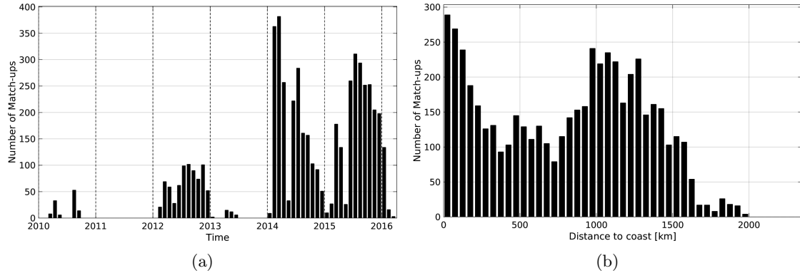
Figure 1: Number of match-ups between Sea mammals and SMOS-L3-CATDS-CECOS-LOCEAN-V2-18DAYS-25KM SSS as a function of time (a) and as function of the distance to coast (b) over the Pacific Ocean Pi-MEP region and for the full satellite product period.
